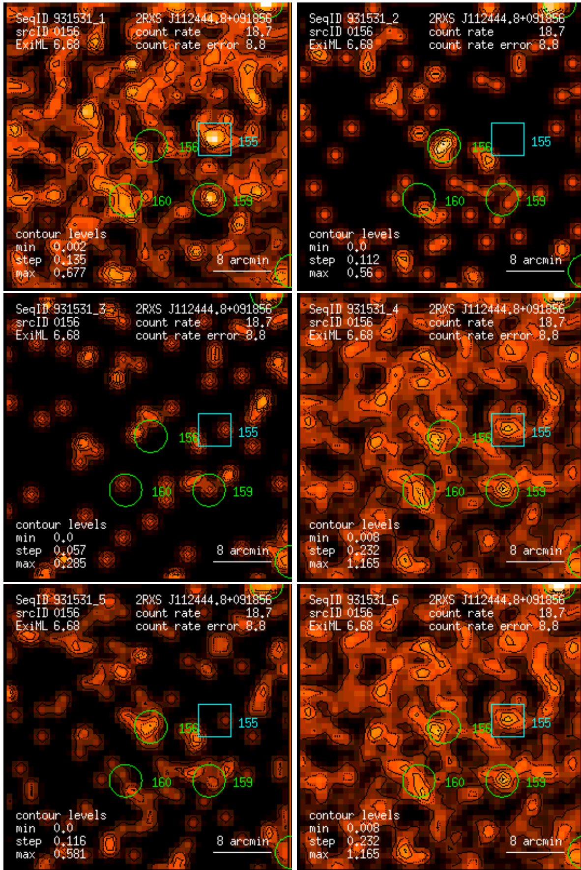
Figure 156: RASS 931531: detection 0156: band rate images, Gaussian filter: (1) PSPC channels 11 – 41, (2) 52 – 90, (3) 91 – 201, (4) 11 – 235, (5) 52 – 201, (6) 11 – 201. Broad band rates in counts/ks. Band rate contour levels in counts/ks/arcmin 2 .
