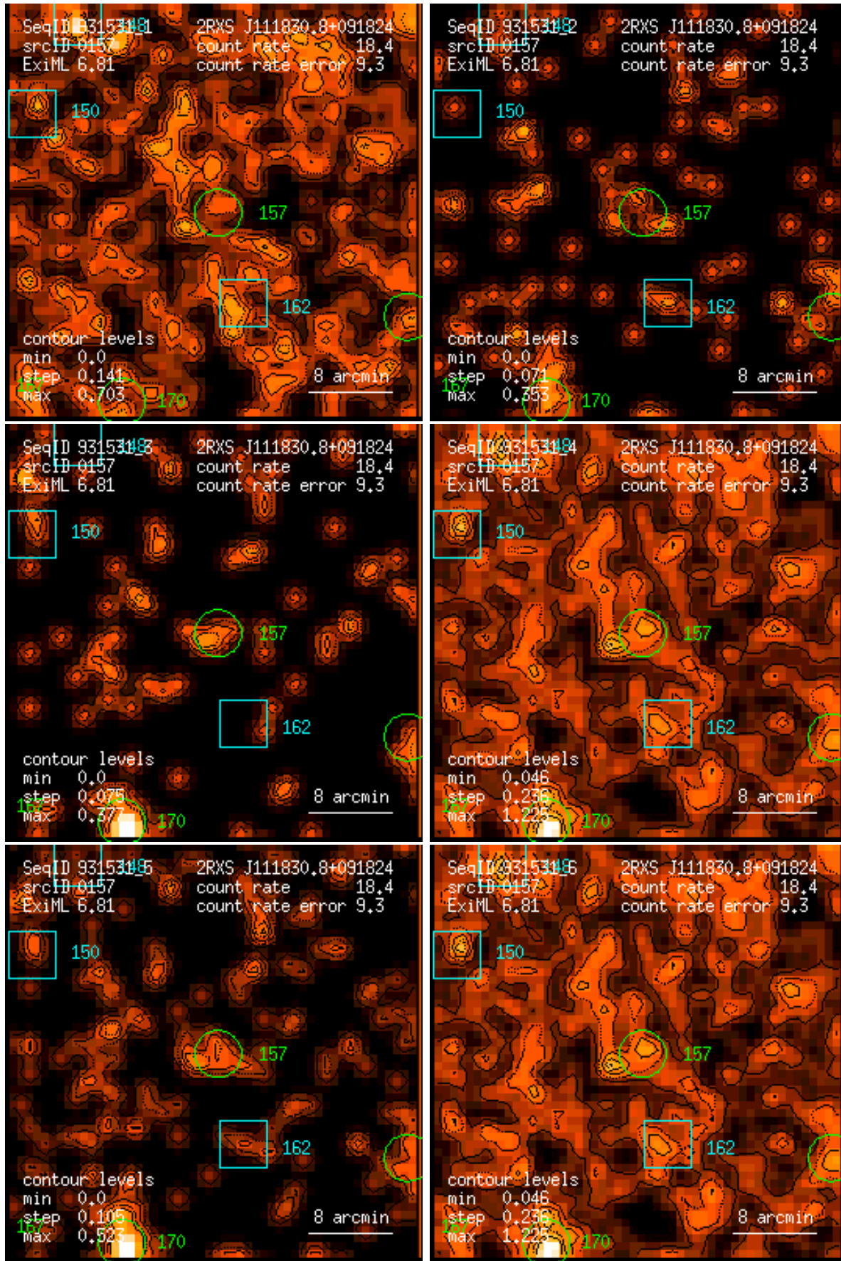
Figure 157: RASS 931531: detection 0157: band rate images, Gaussian filter: (1) PSPC channels 11 – 41, (2) 52 – 90, (3) 91 – 201, (4) 11 – 235, (5) 52 – 201, (6) 11 – 201. Broad band rates in counts/ks. Band rate contour levels in counts/ks/arcmin 2 .
