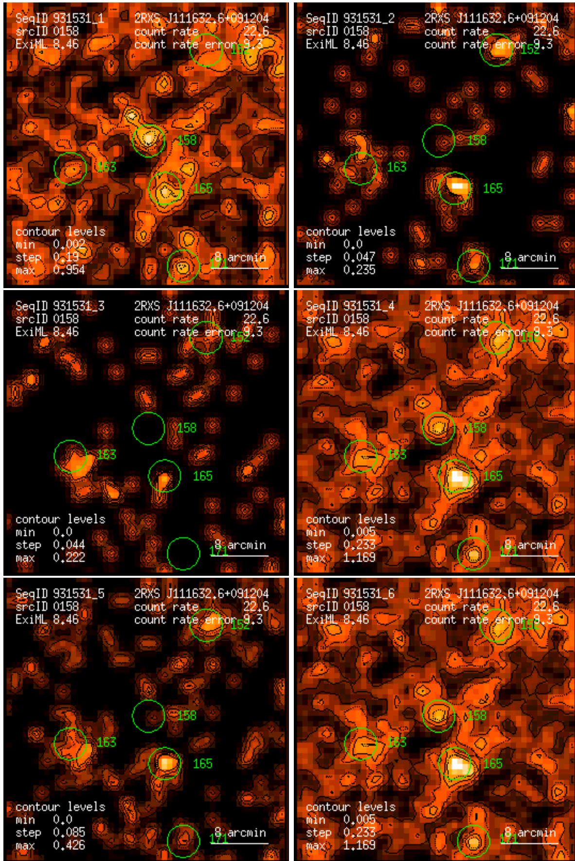
Figure 158: RASS 931531: detection 0158: band rate images, Gaussian filter: (1) PSPC channels 11 – 41, (2) 52 – 90, (3) 91 – 201, (4) 11 – 235, (5) 52 – 201, (6) 11 – 201. Broad band rates in counts/ks. Band rate contour levels in counts/ks/arcmin 2 .
