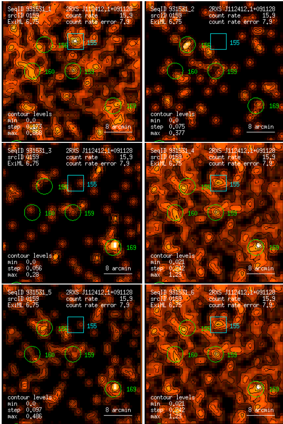
Figure 159: RASS 931531: detection 0159: band rate images, Gaussian filter: (1) PSPC channels 11 – 41, (2) 52 – 90, (3) 91 – 201, (4) 11 – 235, (5) 52 – 201, (6) 11 – 201. Broad band rates in counts/ks. Band rate contour levels in counts/ks/arcmin 2 .
