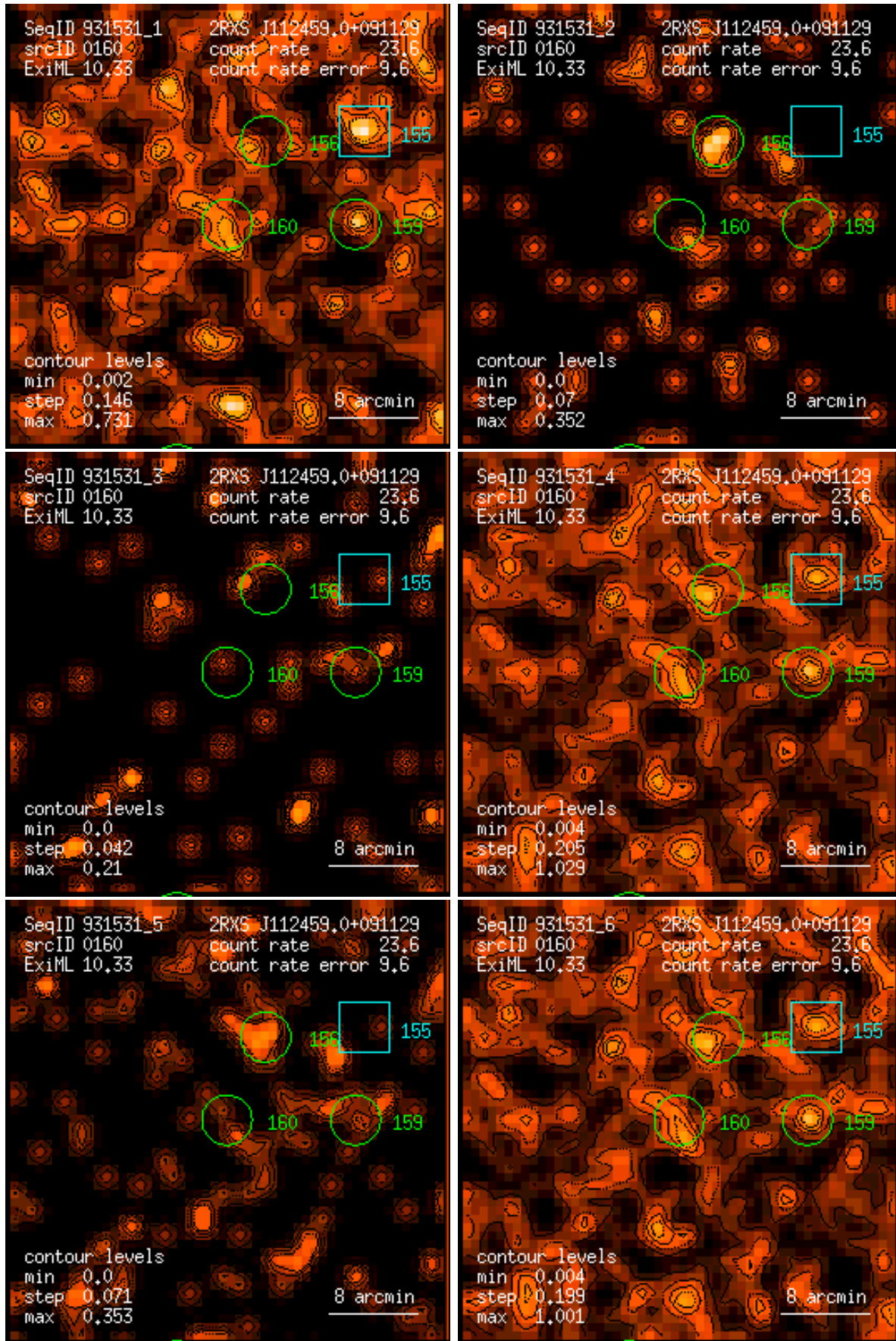
Figure 160: RASS 931531: detection 0160: band rate images, Gaussian filter: (1) PSPC channels 11 – 41, (2) 52 – 90, (3) 91 – 201, (4) 11 – 235, (5) 52 – 201, (6) 11 – 201. Broad band rates in counts/ks. Band rate contour levels in counts/ks/arcmin 2 .
