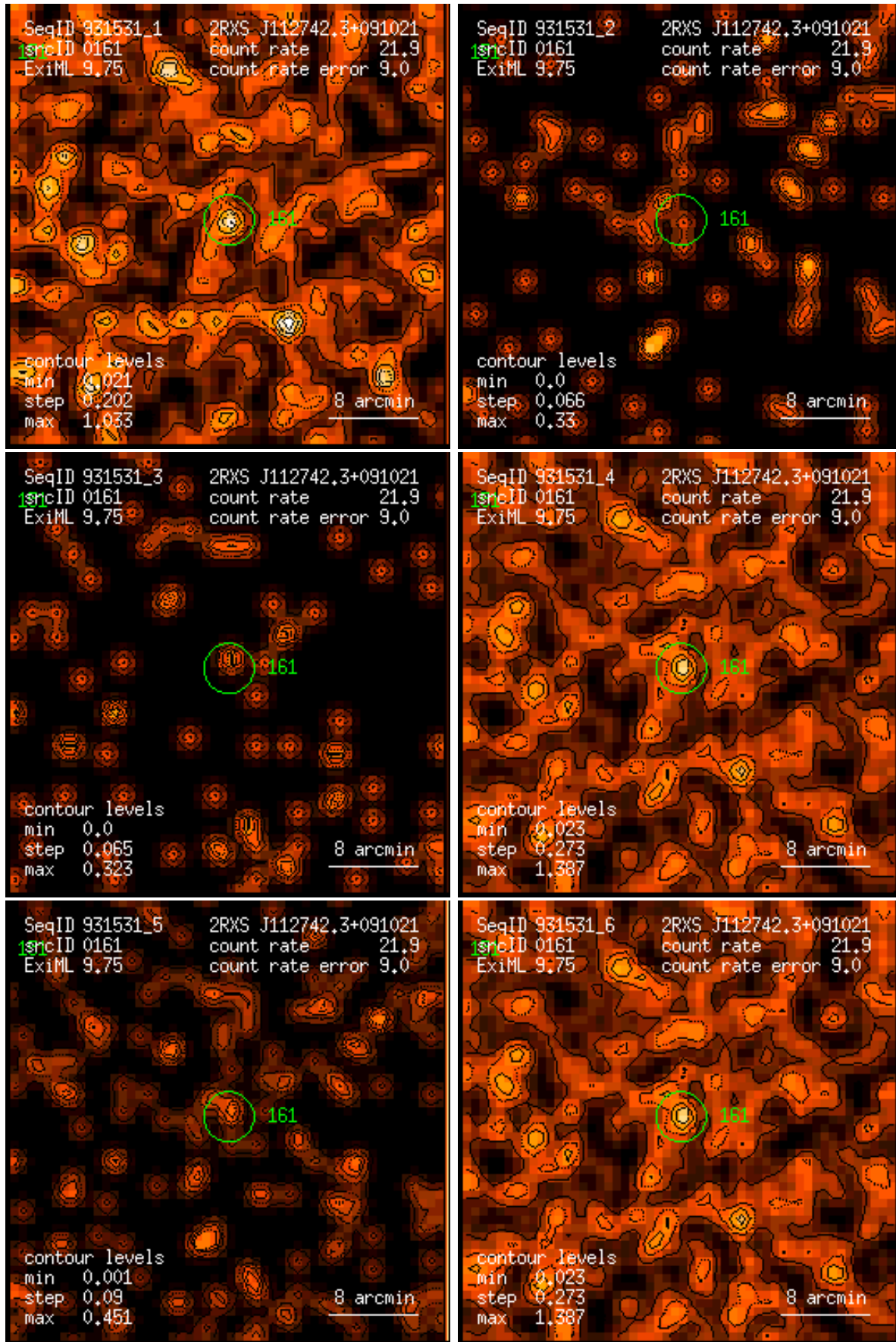
Figure 161: RASS 931531: detection 0161: band rate images, Gaussian filter: (1) PSPC channels 11 – 41, (2) 52 – 90, (3) 91 – 201, (4) 11 – 235, (5) 52 – 201, (6) 11 – 201. Broad band rates in counts/ks. Band rate contour levels in counts/ks/arcmin 2 .
