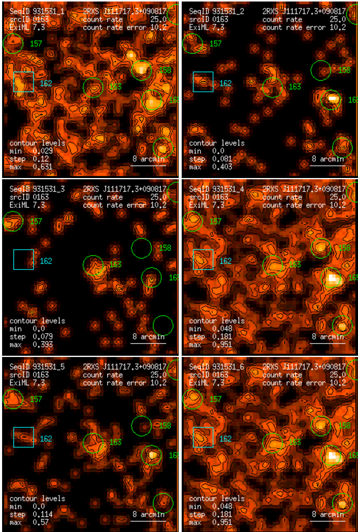
Figure 163: RASS 931531: detection 0163: band rate images, Gaussian filter: (1) PSPC channels 11 – 41, (2) 52 – 90, (3) 91 – 201, (4) 11 – 235, (5) 52 – 201, (6) 11 – 201. Broad band rates in counts/ks. Band rate contour levels in counts/ks/arcmin 2 .
