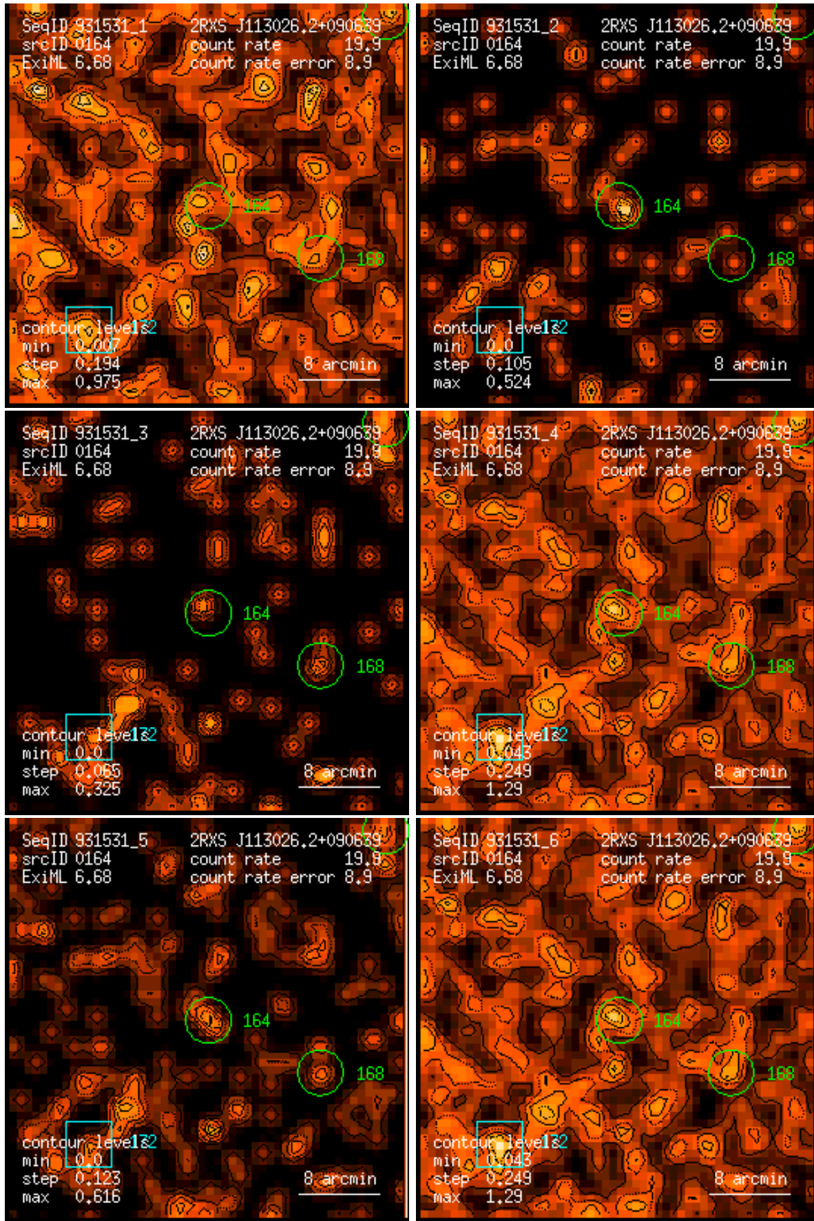
Figure 164: RASS 931531: detection 0164: band rate images, Gaussian filter: (1) PSPC channels 11 – 41, (2) 52 – 90, (3) 91 – 201, (4) 11 – 235, (5) 52 – 201, (6) 11 – 201. Broad band rates in counts/ks. Band rate contour levels in counts/ks/arcmin 2 .
