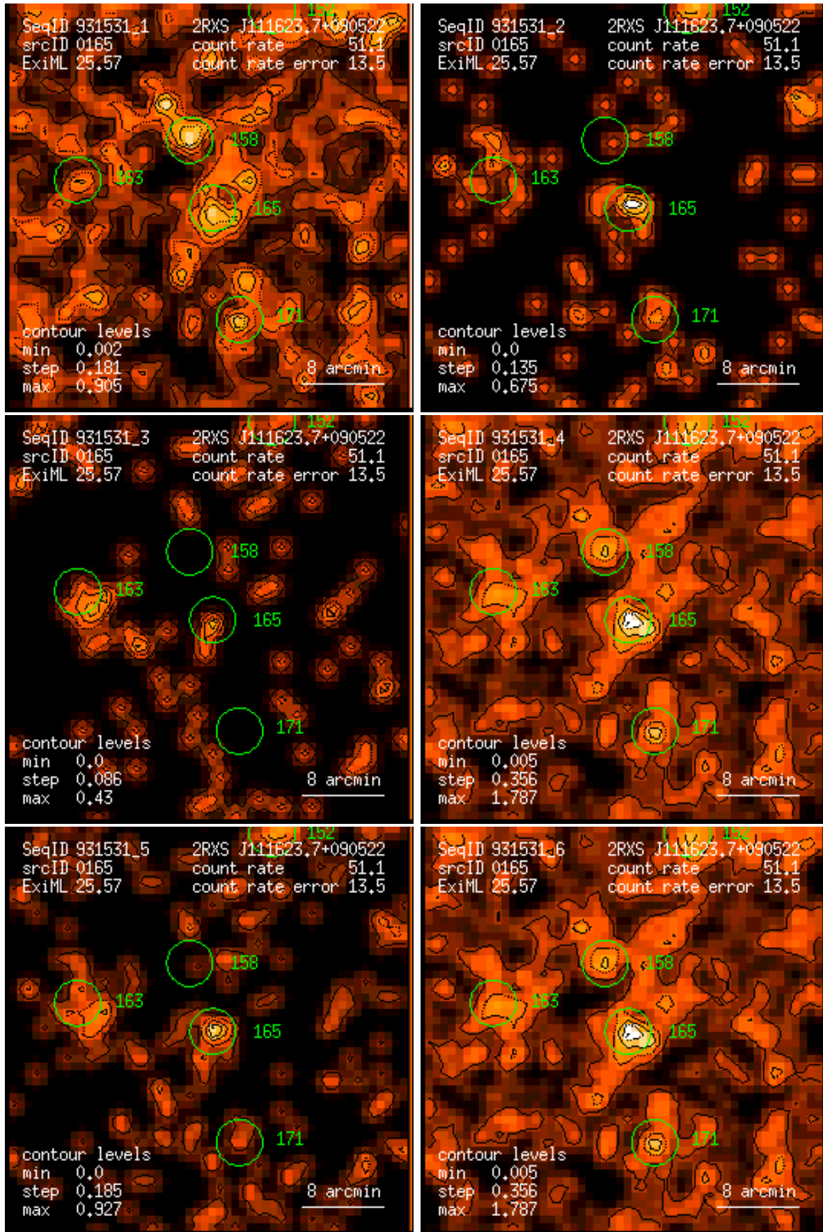
Figure 165: RASS 931531: detection 0165: band rate images, Gaussian filter: (1) PSPC channels 11 – 41, (2) 52 – 90, (3) 91 – 201, (4) 11 – 235, (5) 52 – 201, (6) 11 – 201. Broad band rates in counts/ks. Band rate contour levels in counts/ks/arcmin 2 .
