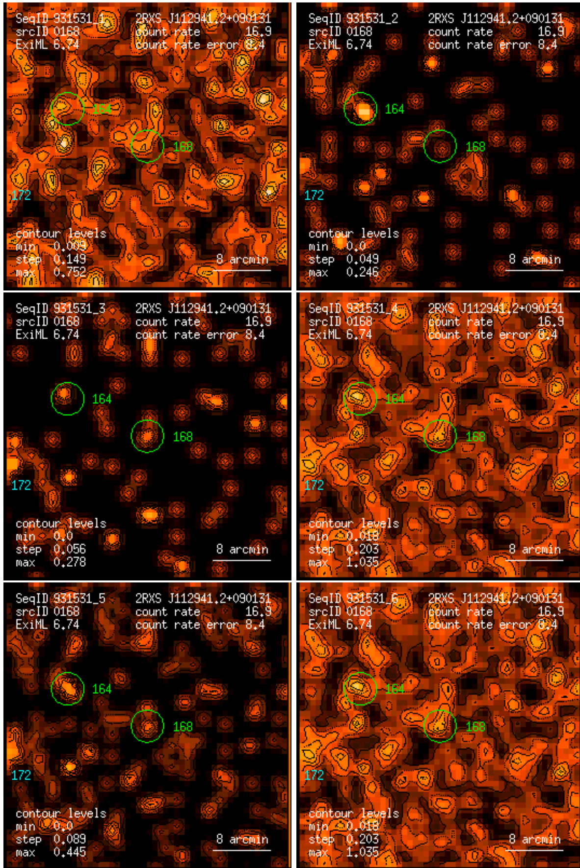
Figure 168: RASS 931531: detection 0168: band rate images, Gaussian filter: (1) PSPC channels 11 – 41, (2) 52 – 90, (3) 91 – 201, (4) 11 – 235, (5) 52 – 201, (6) 11 – 201. Broad band rates in counts/ks. Band rate contour levels in counts/ks/arcmin 2 .
