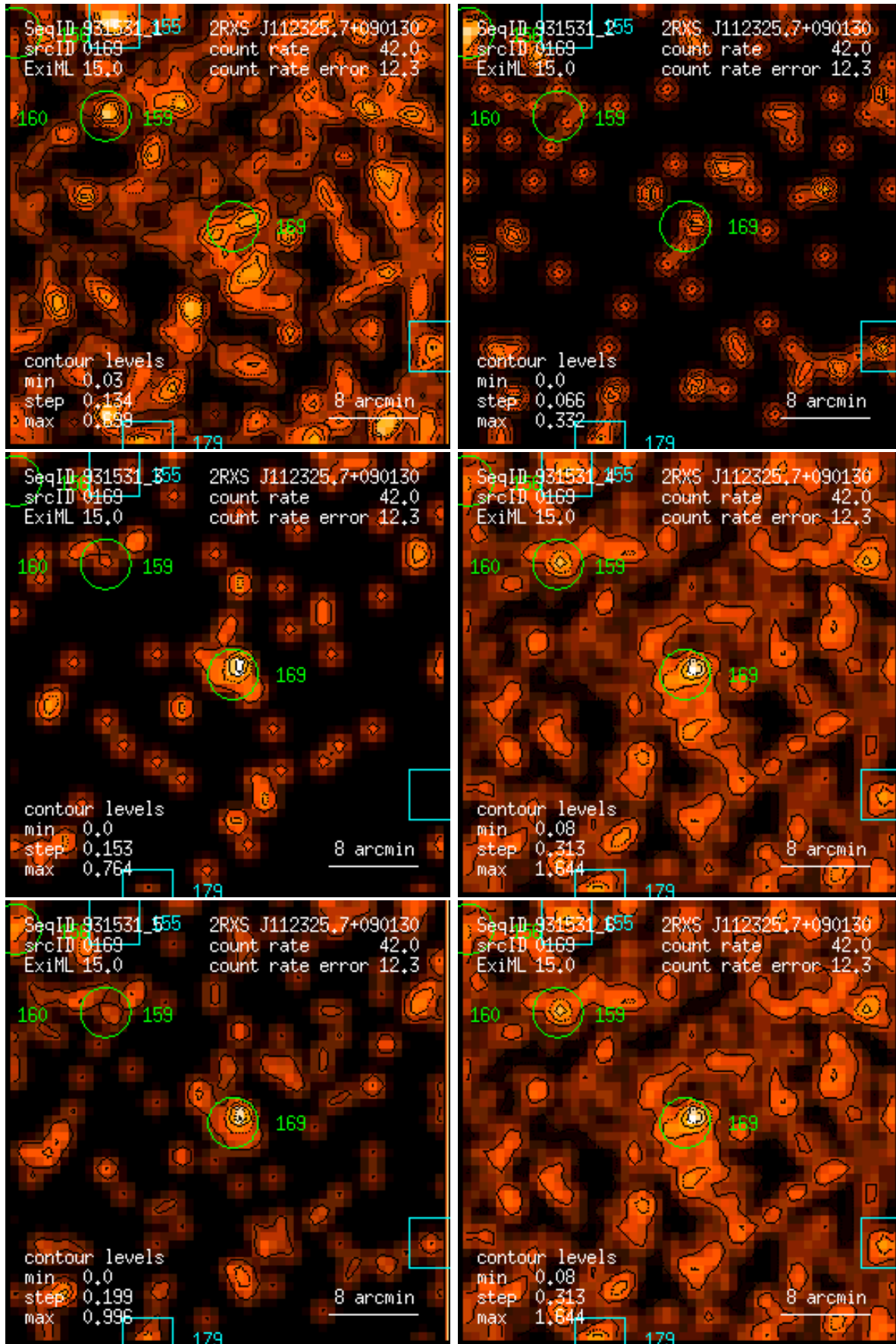
Figure 169: RASS 931531: detection 0169: band rate images, Gaussian filter: (1) PSPC channels 11 – 41, (2) 52 – 90, (3) 91 – 201, (4) 11 – 235, (5) 52 – 201, (6) 11 – 201. Broad band rates in counts/ks. Band rate contour levels in counts/ks/arcmin 2 .
