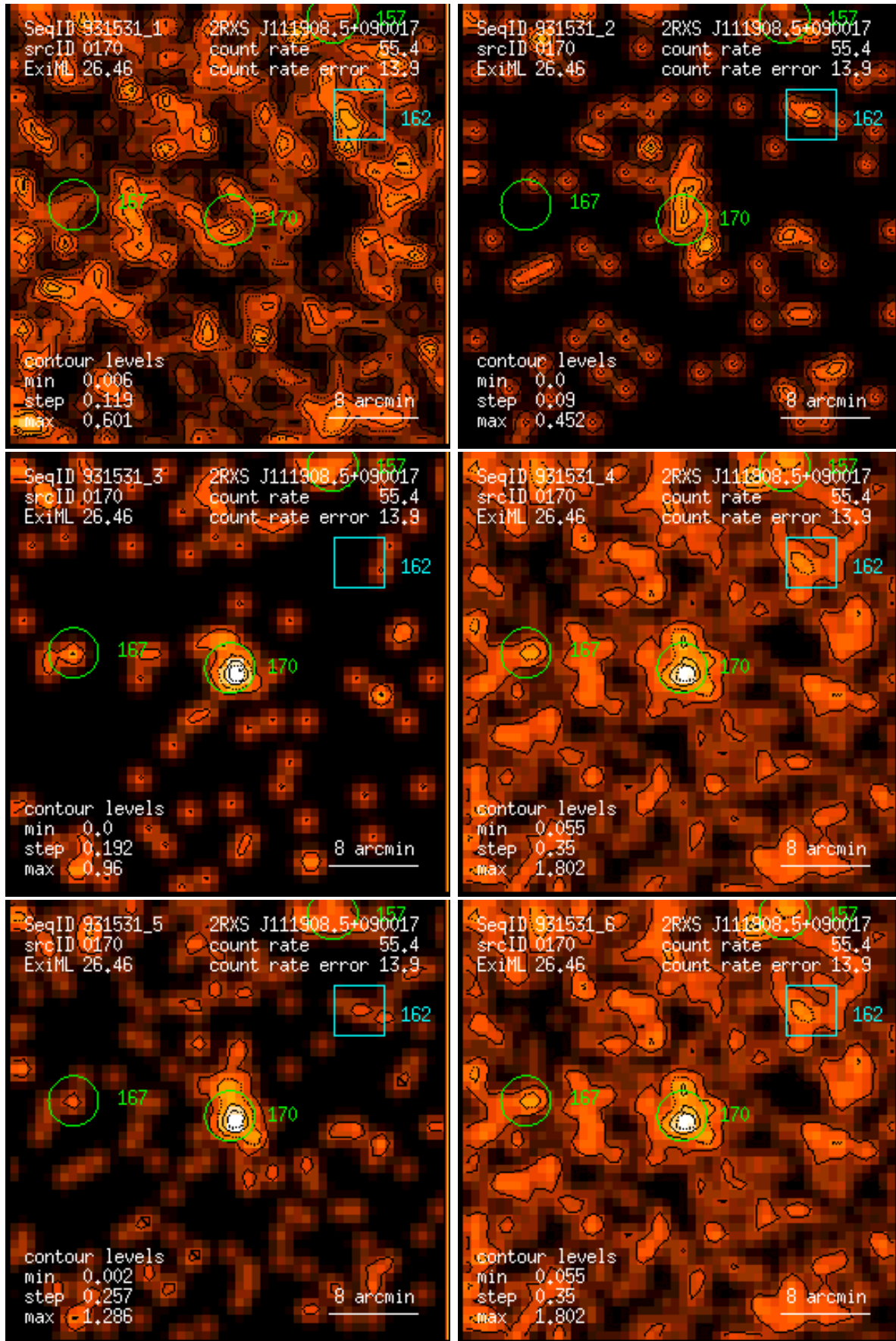
Figure 170: RASS 931531: detection 0170: band rate images, Gaussian filter: (1) PSPC channels 11 – 41, (2) 52 – 90, (3) 91 – 201, (4) 11 – 235, (5) 52 – 201, (6) 11 – 201. Broad band rates in counts/ks. Band rate contour levels in counts/ks/arcmin 2 .
