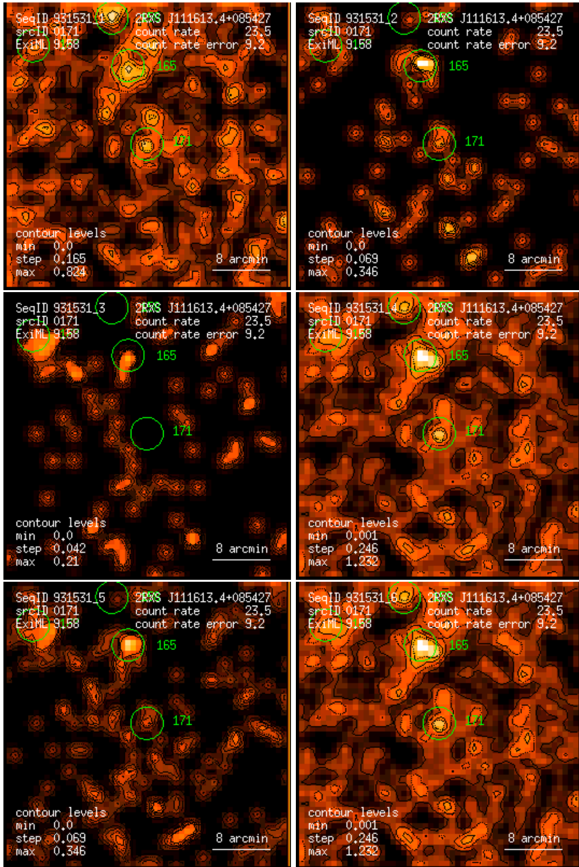
Figure 171: RASS 931531: detection 0171: band rate images, Gaussian filter: (1) PSPC channels 11 – 41, (2) 52 – 90, (3) 91 – 201, (4) 11 – 235, (5) 52 – 201, (6) 11 – 201. Broad band rates in counts/ks. Band rate contour levels in counts/ks/arcmin 2 .
