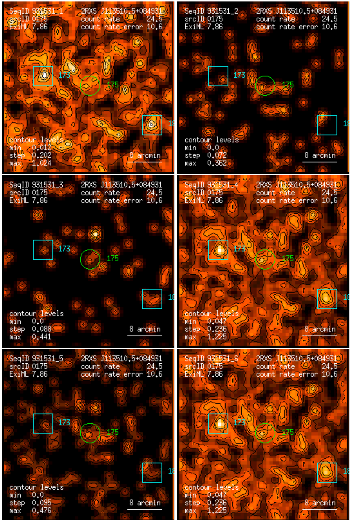
Figure 175: RASS 931531: detection 0175: band rate images, Gaussian filter: (1) PSPC channels 11 – 41, (2) 52 – 90, (3) 91 – 201, (4) 11 – 235, (5) 52 – 201, (6) 11 – 201. Broad band rates in counts/ks. Band rate contour levels in counts/ks/arcmin 2 .
