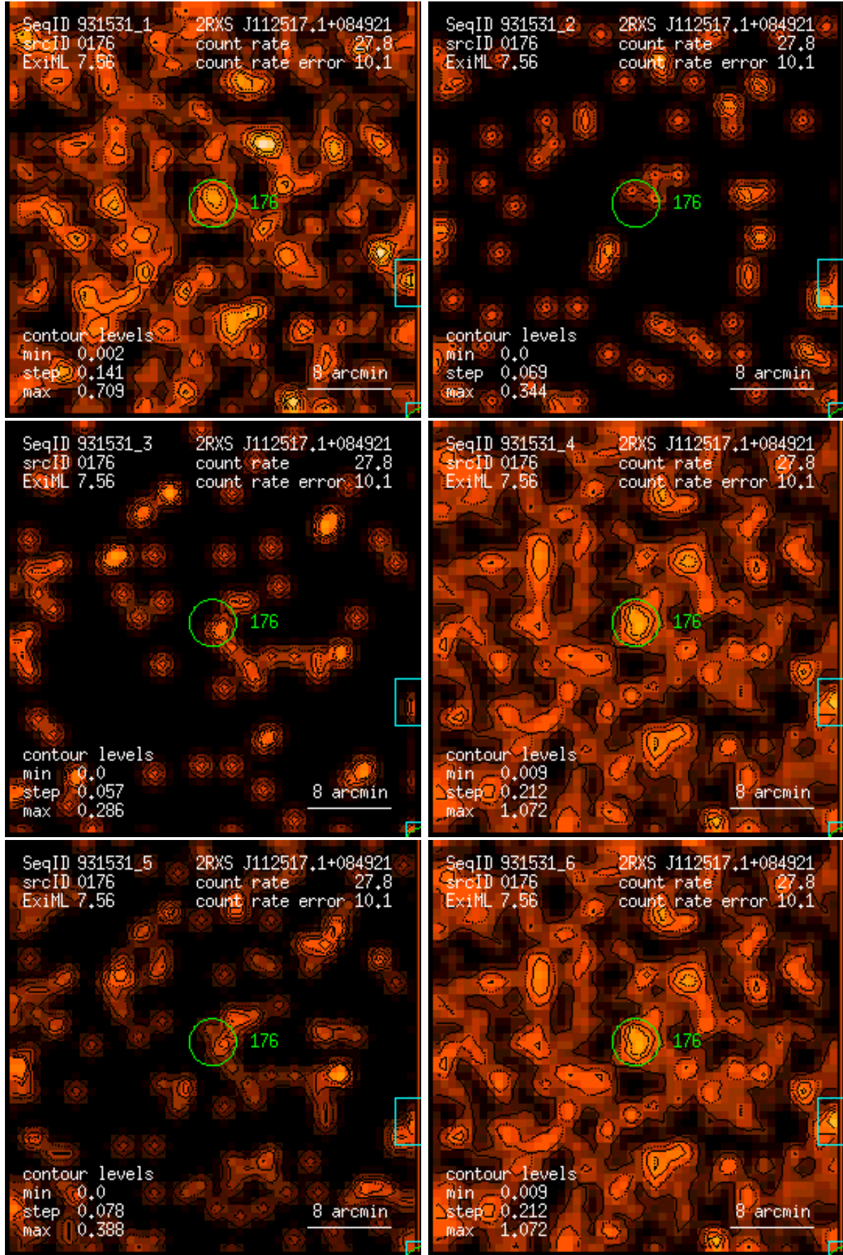
Figure 176: RASS 931531: detection 0176: band rate images, Gaussian filter: (1) PSPC channels 11 – 41, (2) 52 – 90, (3) 91 – 201, (4) 11 – 235, (5) 52 – 201, (6) 11 – 201. Broad band rates in counts/ks. Band rate contour levels in counts/ks/arcmin 2 .
