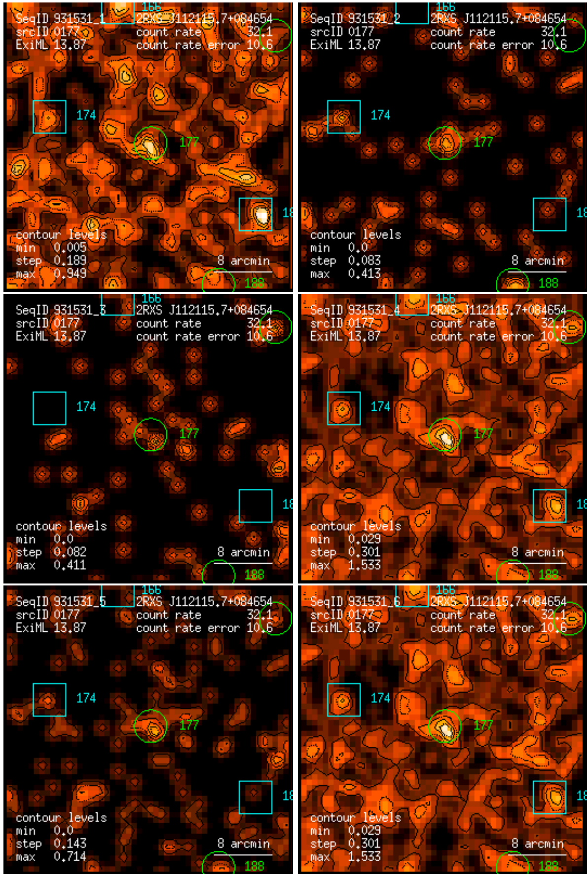
Figure 177: RASS 931531: detection 0177: band rate images, Gaussian filter: (1) PSPC channels 11 – 41, (2) 52 – 90, (3) 91 – 201, (4) 11 – 235, (5) 52 – 201, (6) 11 – 201. Broad band rates in counts/ks. Band rate contour levels in counts/ks/arcmin 2 .
