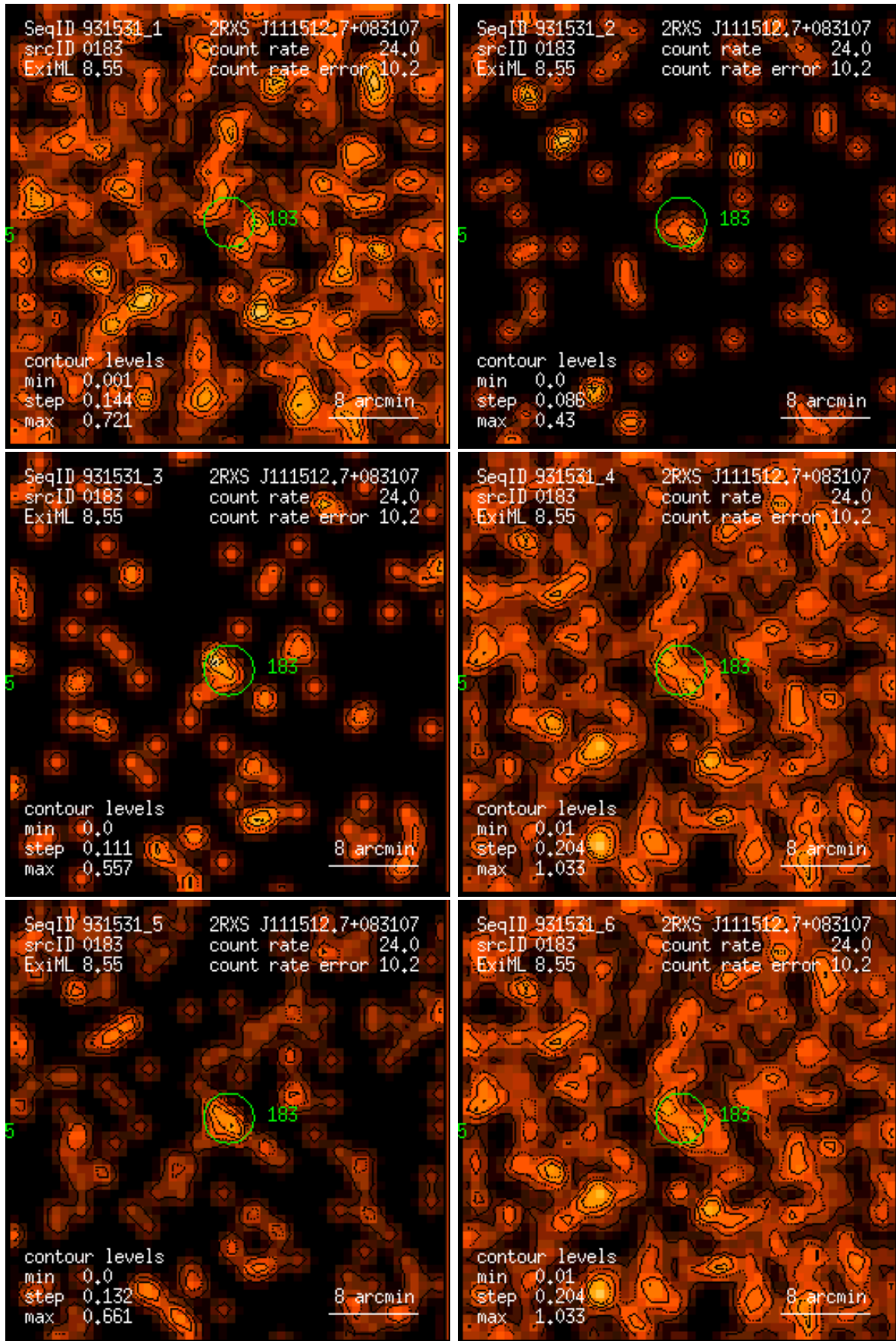
Figure 183: RASS 931531: detection 0183: band rate images, Gaussian filter: (1) PSPC channels 11 – 41, (2) 52 – 90, (3) 91 – 201, (4) 11 – 235, (5) 52 – 201, (6) 11 – 201. Broad band rates in counts/ks. Band rate contour levels in counts/ks/arcmin 2 .
