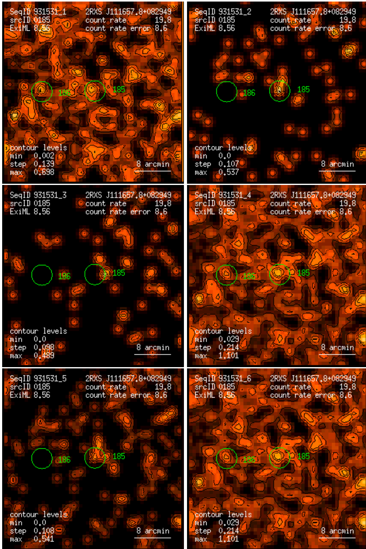
Figure 185: RASS 931531: detection 0185: band rate images, Gaussian filter: (1) PSPC channels 11 – 41, (2) 52 – 90, (3) 91 – 201, (4) 11 – 235, (5) 52 – 201, (6) 11 – 201. Broad band rates in counts/ks. Band rate contour levels in counts/ks/arcmin 2 .
