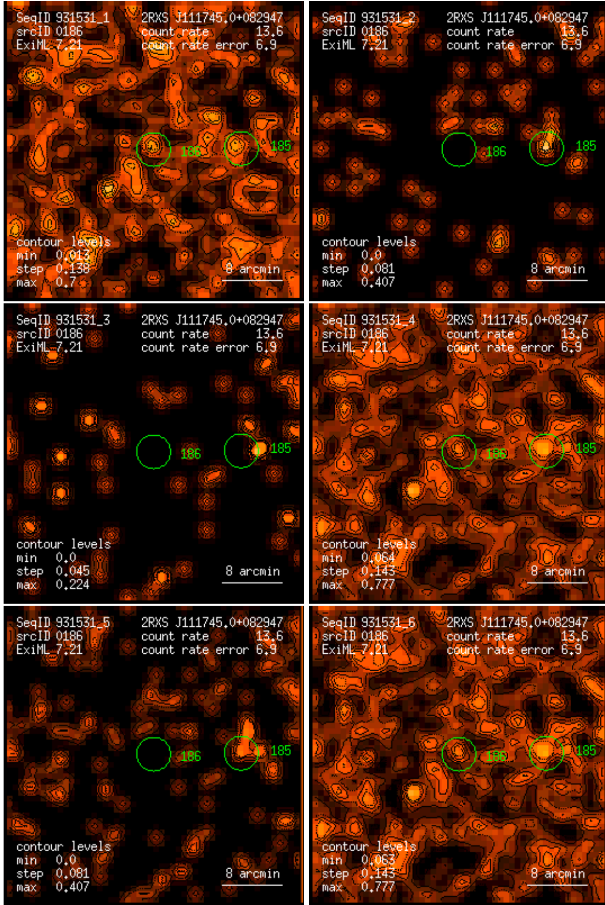
Figure 186: RASS 931531: detection 0186: band rate images, Gaussian filter: (1) PSPC channels 11 – 41, (2) 52 – 90, (3) 91 – 201, (4) 11 – 235, (5) 52 – 201, (6) 11 – 201. Broad band rates in counts/ks. Band rate contour levels in counts/ks/arcmin 2 .
