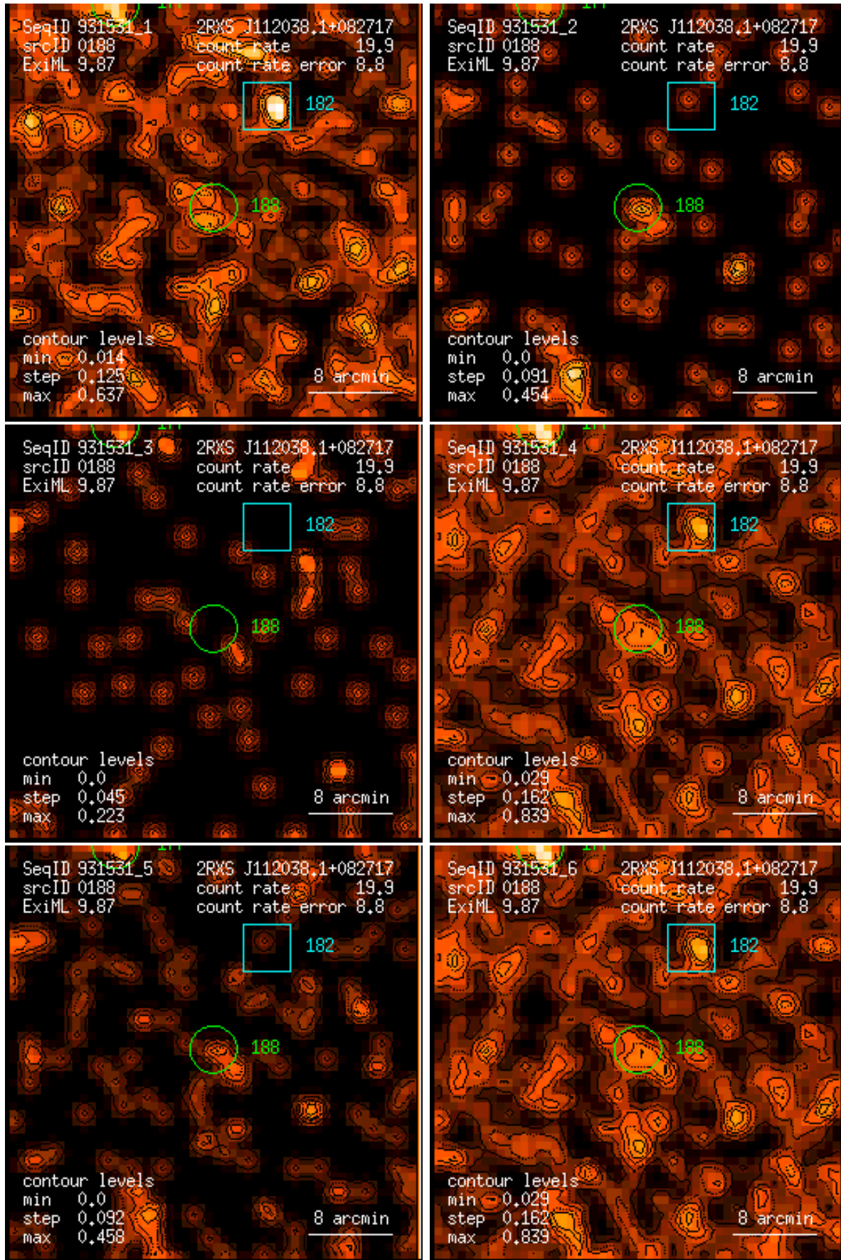
Figure 188: RASS 931531: detection 0188: band rate images, Gaussian filter: (1) PSPC channels 11 – 41, (2) 52 – 90, (3) 91 – 201, (4) 11 – 235, (5) 52 – 201, (6) 11 – 201. Broad band rates in counts/ks. Band rate contour levels in counts/ks/arcmin 2 .
