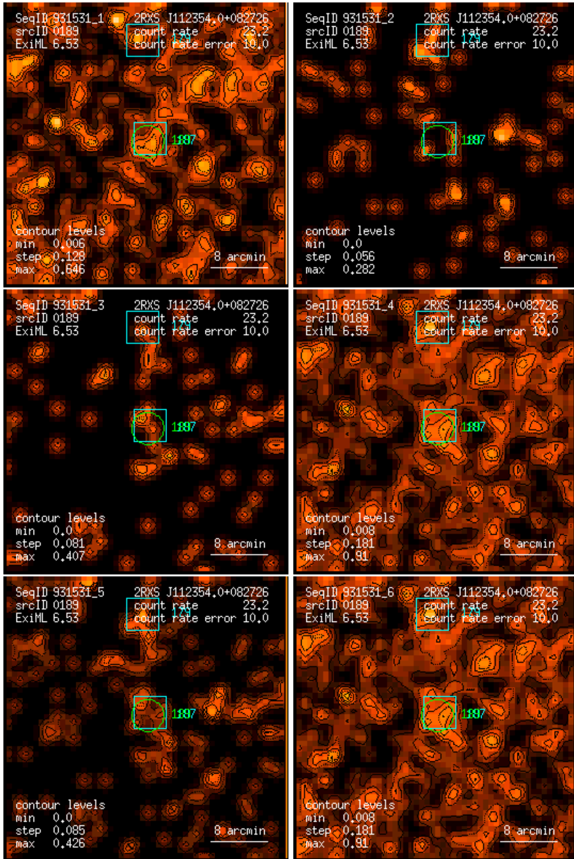
Figure 189: RASS 931531: detection 0189: band rate images, Gaussian filter: (1) PSPC channels 11 – 41, (2) 52 – 90, (3) 91 – 201, (4) 11 – 235, (5) 52 – 201, (6) 11 – 201. Broad band rates in counts/ks. Band rate contour levels in counts/ks/arcmin 2 .
