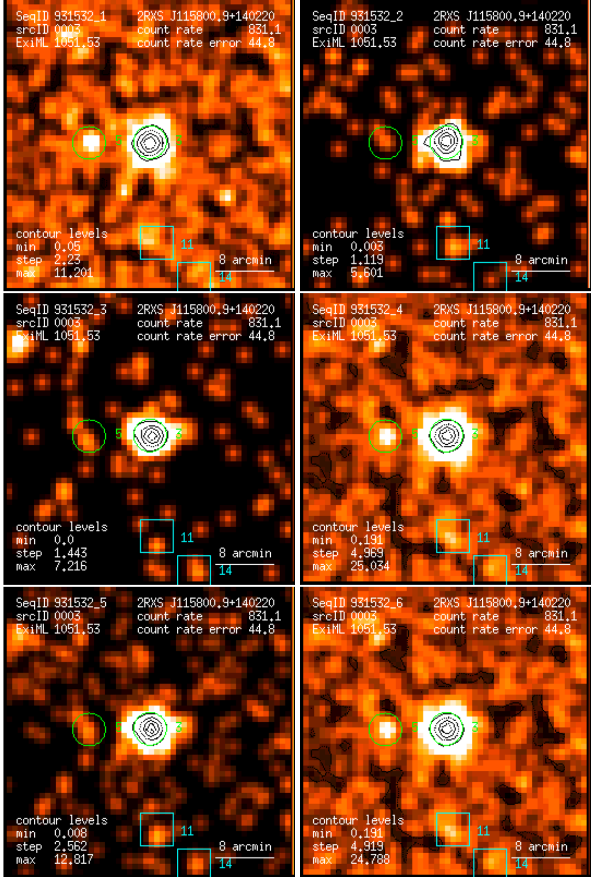
Figure 3: RASS 931532: detection 0003: band rate images, Gaussian filter: (1) PSPC channels 11 – 41, (2) 52 – 90, (3) 91 – 201, (4) 11 – 235, (5) 52 – 201, (6) 11 – 201. Broad band rates in counts/ks. Band rate contour levels in counts/ks/arcmin 2 .
