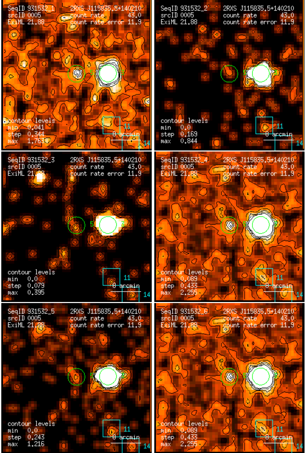
Figure 5: RASS 931532: detection 0005: band rate images, Gaussian filter: (1) PSPC channels 11 – 41, (2) 52 – 90, (3) 91 – 201, (4) 11 – 235, (5) 52 – 201, (6) 11 – 201. Broad band rates in counts/ks. Band rate contour levels in counts/ks/arcmin 2 .
