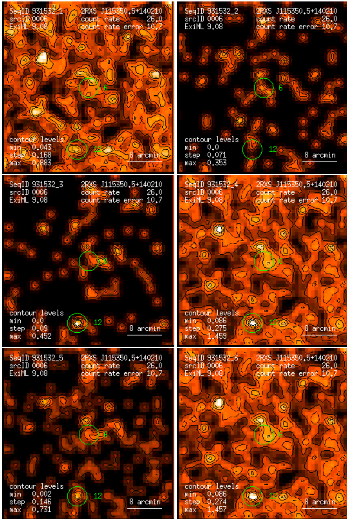
Figure 6: RASS 931532: detection 0006: band rate images, Gaussian filter: (1) PSPC channels 11 – 41, (2) 52 – 90, (3) 91 – 201, (4) 11 – 235, (5) 52 – 201, (6) 11 – 201. Broad band rates in counts/ks. Band rate contour levels in counts/ks/arcmin 2 .
