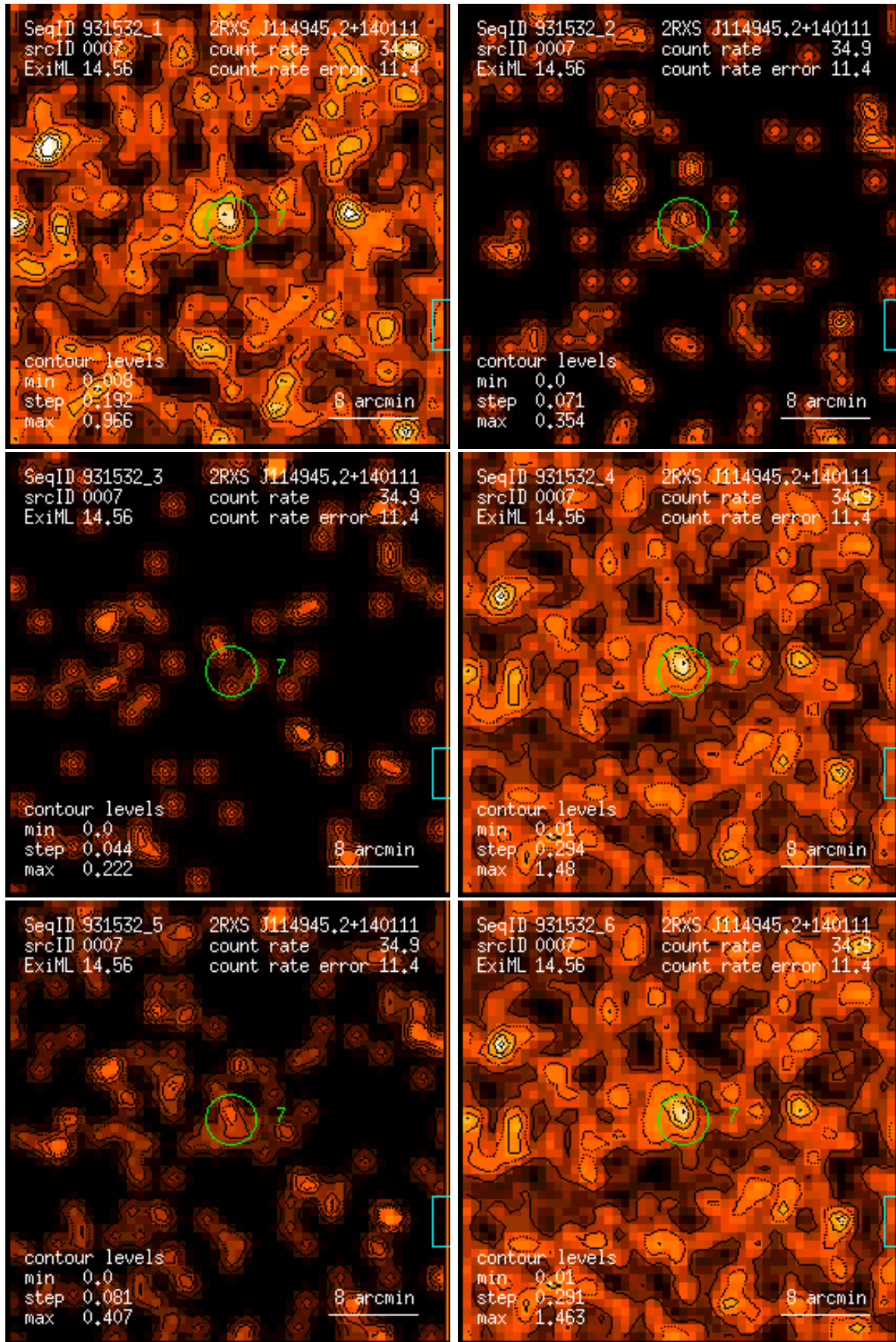
Figure 7: RASS 931532: detection 0007: band rate images, Gaussian filter: (1) PSPC channels 11 – 41, (2) 52 – 90, (3) 91 – 201, (4) 11 – 235, (5) 52 – 201, (6) 11 – 201. Broad band rates in counts/ks. Band rate contour levels in counts/ks/arcmin 2 .
