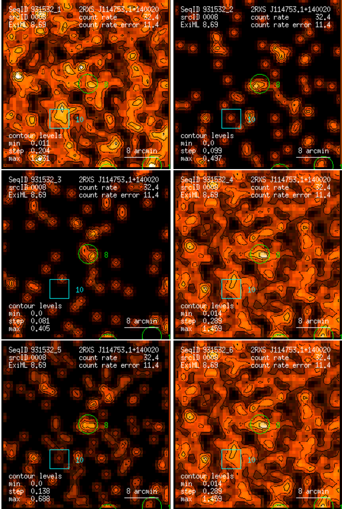
Figure 8: RASS 931532: detection 0008: band rate images, Gaussian filter: (1) PSPC channels 11 – 41, (2) 52 – 90, (3) 91 – 201, (4) 11 – 235, (5) 52 – 201, (6) 11 – 201. Broad band rates in counts/ks. Band rate contour levels in counts/ks/arcmin 2 .
