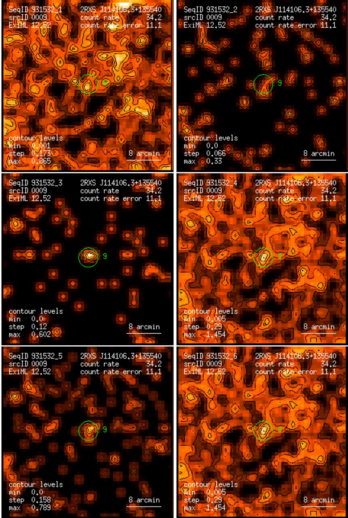
Figure 9: RASS 931532: detection 0009: band rate images, Gaussian filter: (1) PSPC channels 11 – 41, (2) 52 – 90, (3) 91 – 201, (4) 11 – 235, (5) 52 – 201, (6) 11 – 201. Broad band rates in counts/ks. Band rate contour levels in counts/ks/arcmin 2 .
