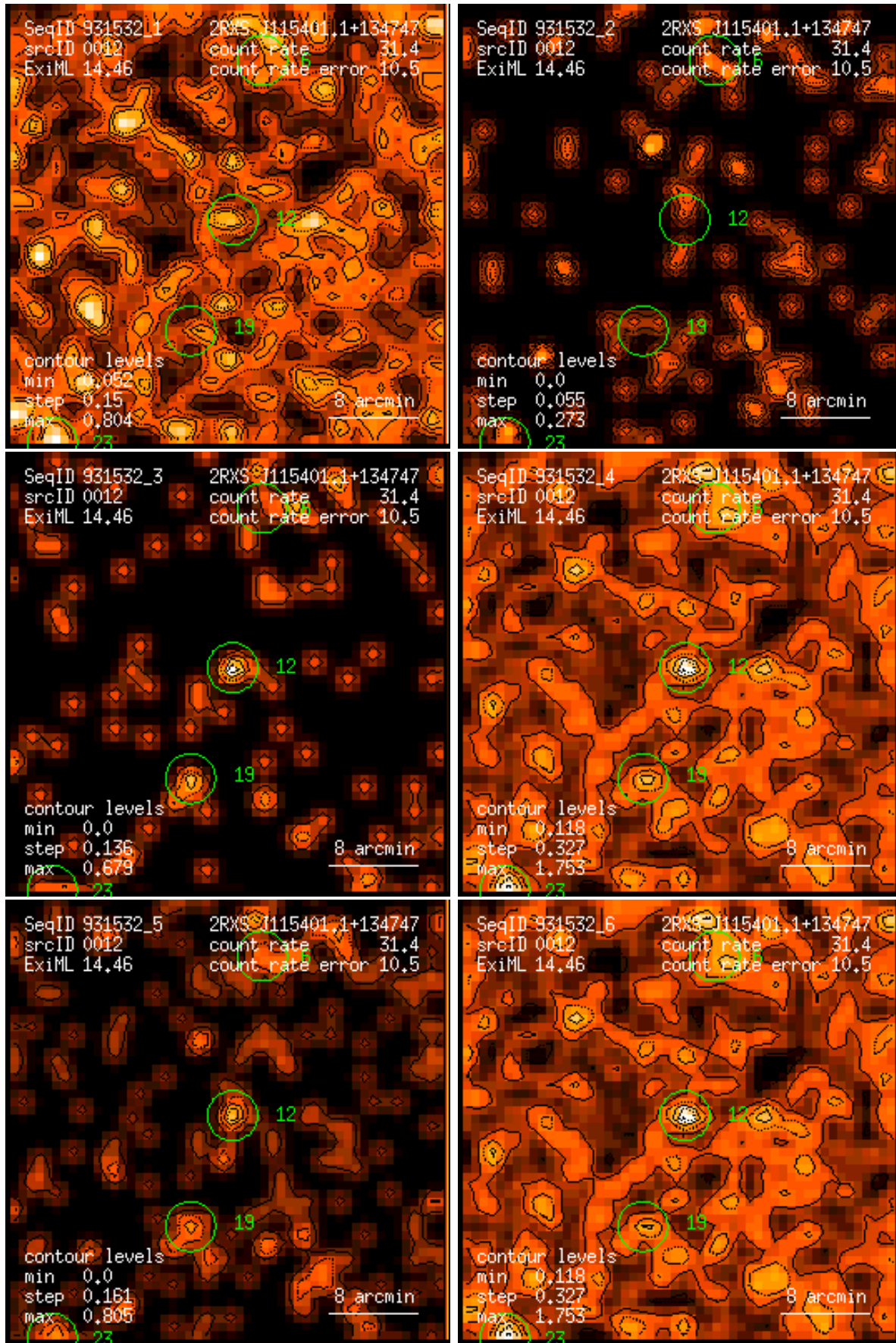
Figure 12: RASS 931532: detection 0012: band rate images, Gaussian filter: (1) PSPC channels 11 – 41, (2) 52 – 90, (3) 91 – 201, (4) 11 – 235, (5) 52 – 201, (6) 11 – 201. Broad band rates in counts/ks. Band rate contour levels in counts/ks/arcmin 2 .
