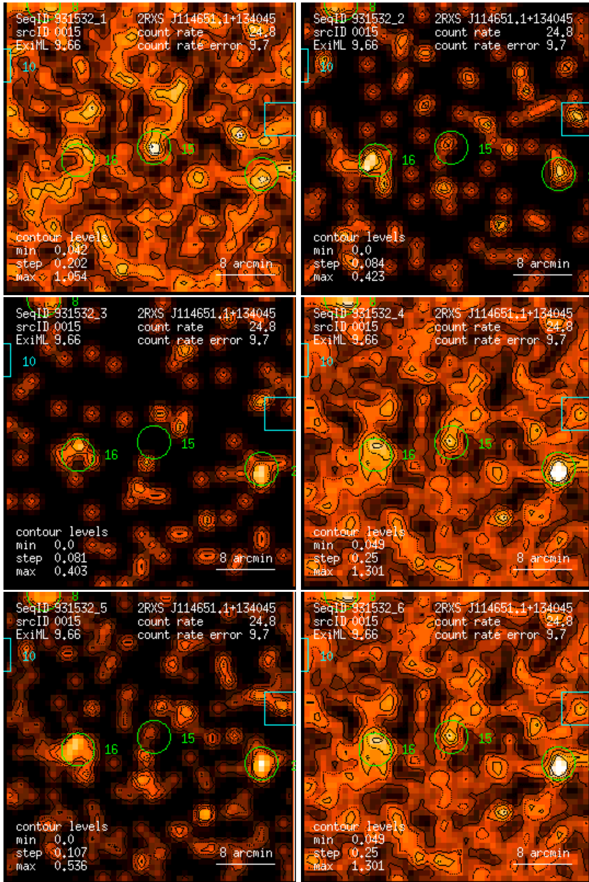
Figure 15: RASS 931532: detection 0015: band rate images, Gaussian filter: (1) PSPC channels 11 – 41, (2) 52 – 90, (3) 91 – 201, (4) 11 – 235, (5) 52 – 201, (6) 11 – 201. Broad band rates in counts/ks. Band rate contour levels in counts/ks/arcmin 2 .
