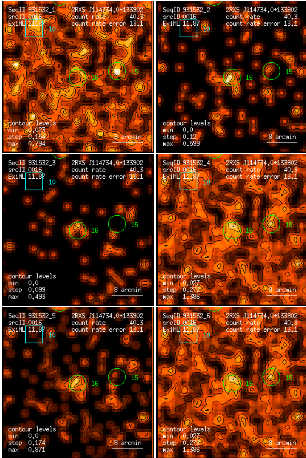
Figure 16: RASS 931532: detection 0016: band rate images, Gaussian filter: (1) PSPC channels 11 – 41, (2) 52 – 90, (3) 91 – 201, (4) 11 – 235, (5) 52 – 201, (6) 11 – 201. Broad band rates in counts/ks. Band rate contour levels in counts/ks/arcmin 2 .
