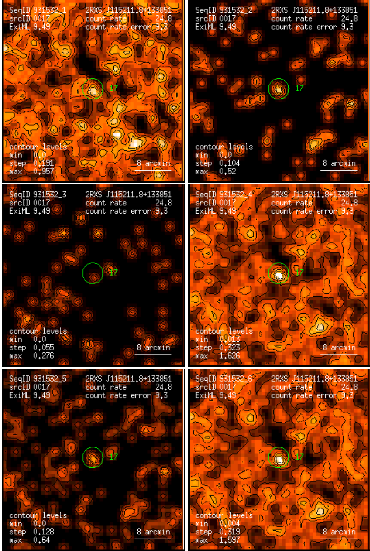
Figure 17: RASS 931532: detection 0017: band rate images, Gaussian filter: (1) PSPC channels 11 – 41, (2) 52 – 90, (3) 91 – 201, (4) 11 – 235, (5) 52 – 201, (6) 11 – 201. Broad band rates in counts/ks. Band rate contour levels in counts/ks/arcmin 2 .
