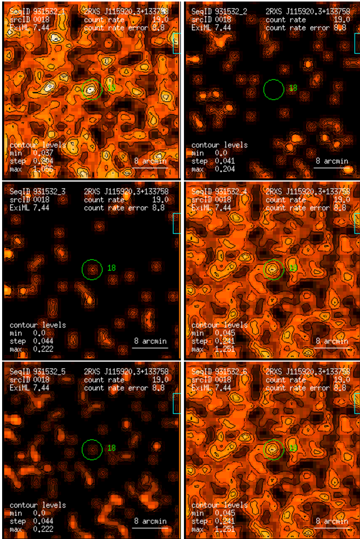
Figure 18: RASS 931532: detection 0018: band rate images, Gaussian filter: (1) PSPC channels 11 – 41, (2) 52 – 90, (3) 91 – 201, (4) 11 – 235, (5) 52 – 201, (6) 11 – 201. Broad band rates in counts/ks. Band rate contour levels in counts/ks/arcmin 2 .
