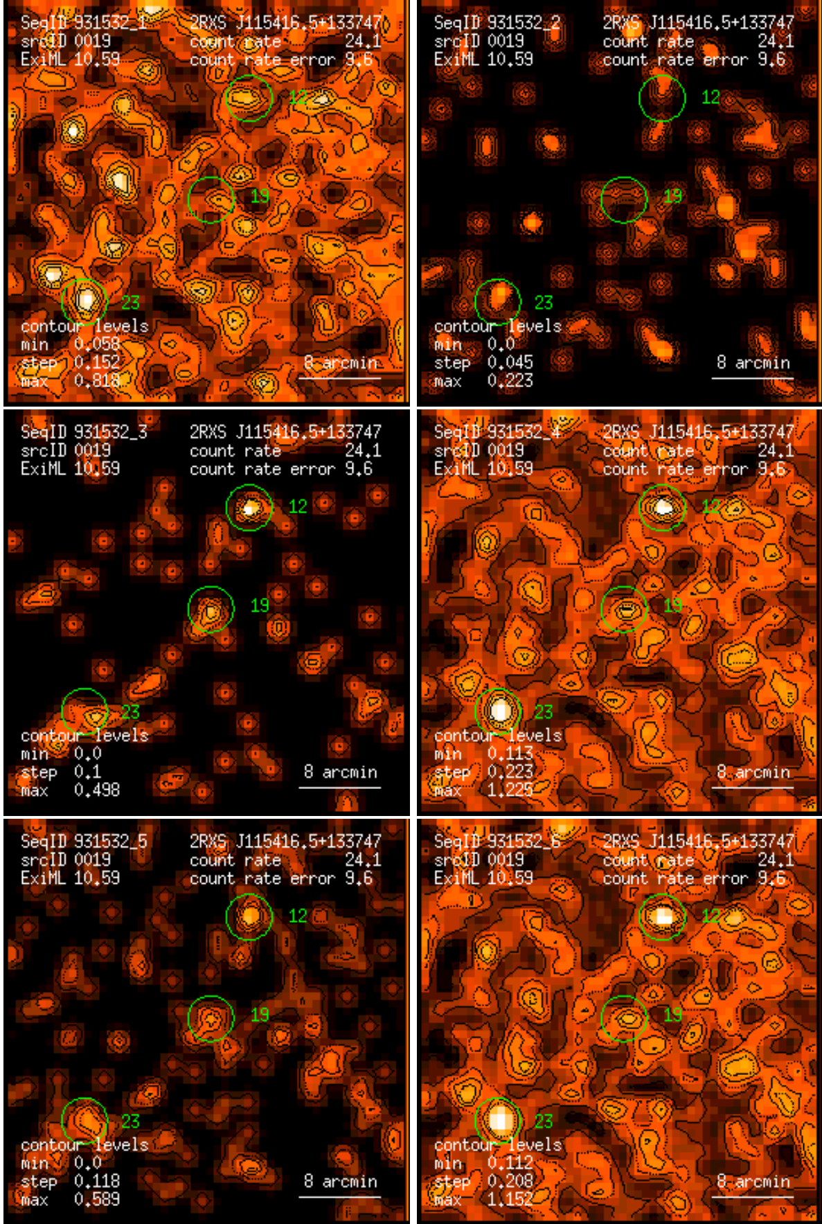
Figure 19: RASS 931532: detection 0019: band rate images, Gaussian filter: (1) PSPC channels 11 – 41, (2) 52 – 90, (3) 91 – 201, (4) 11 – 235, (5) 52 – 201, (6) 11 – 201. Broad band rates in counts/ks. Band rate contour levels in counts/ks/arcmin 2 .
