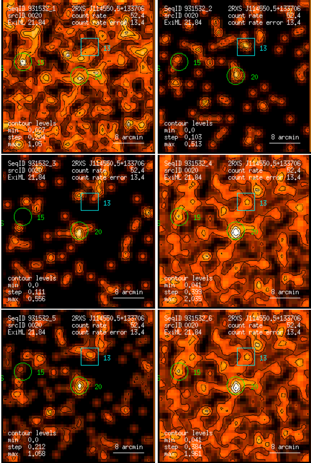
Figure 20: RASS 931532: detection 0020: band rate images, Gaussian filter: (1) PSPC channels 11 – 41, (2) 52 – 90, (3) 91 – 201, (4) 11 – 235, (5) 52 – 201, (6) 11 – 201. Broad band rates in counts/ks. Band rate contour levels in counts/ks/arcmin 2 .
