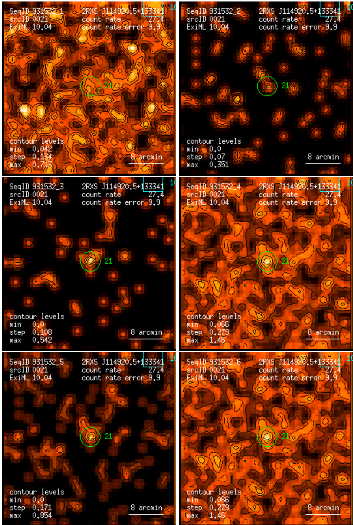
Figure 21: RASS 931532: detection 0021: band rate images, Gaussian filter: (1) PSPC channels 11 – 41, (2) 52 – 90, (3) 91 – 201, (4) 11 – 235, (5) 52 – 201, (6) 11 – 201. Broad band rates in counts/ks. Band rate contour levels in counts/ks/arcmin 2 .
