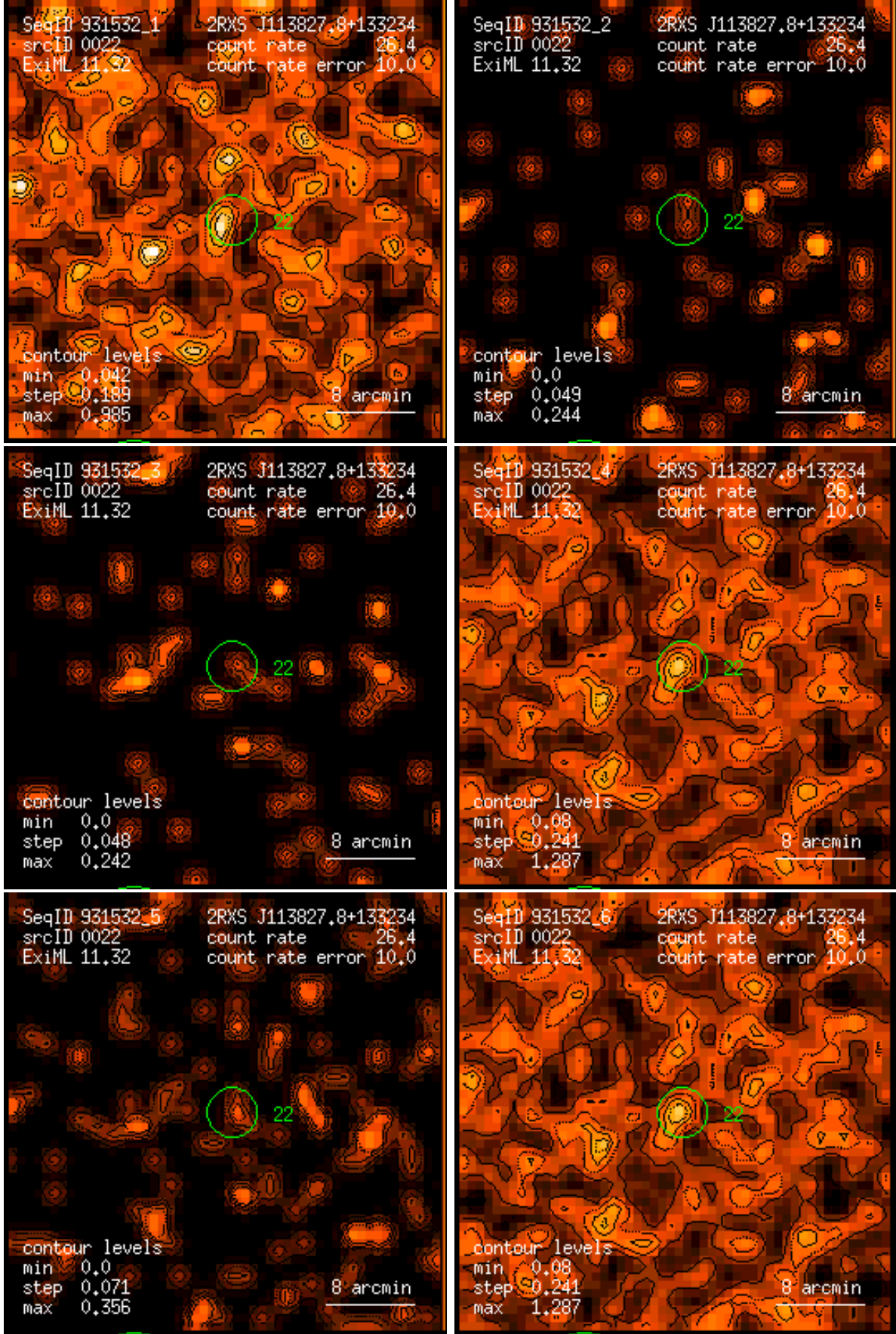
Figure 22: RASS 931532: detection 0022: band rate images, Gaussian filter: (1) PSPC channels 11 – 41, (2) 52 – 90, (3) 91 – 201, (4) 11 – 235, (5) 52 – 201, (6) 11 – 201. Broad band rates in counts/ks. Band rate contour levels in counts/ks/arcmin 2 .
