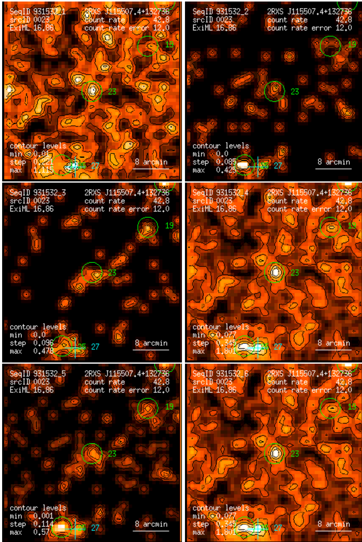
Figure 23: RASS 931532: detection 0023: band rate images, Gaussian filter: (1) PSPC channels 11 – 41, (2) 52 – 90, (3) 91 – 201, (4) 11 – 235, (5) 52 – 201, (6) 11 – 201. Broad band rates in counts/ks. Band rate contour levels in counts/ks/arcmin 2 .
