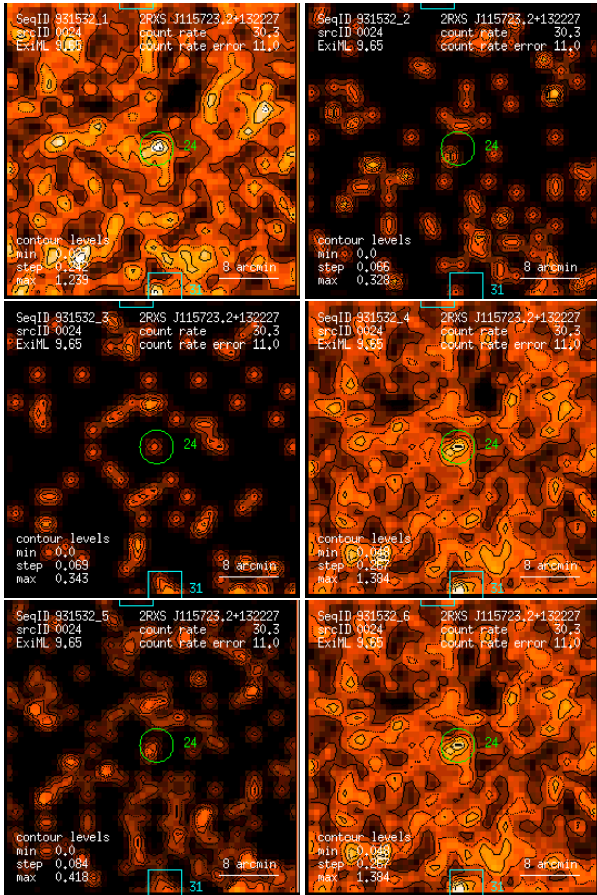
Figure 24: RASS 931532: detection 0024: band rate images, Gaussian filter: (1) PSPC channels 11 – 41, (2) 52 – 90, (3) 91 – 201, (4) 11 – 235, (5) 52 – 201, (6) 11 – 201. Broad band rates in counts/ks. Band rate contour levels in counts/ks/arcmin 2 .
