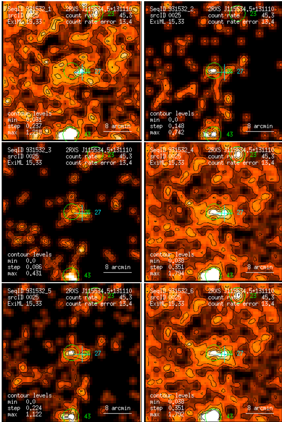
Figure 25: RASS 931532: detection 0025: band rate images, Gaussian filter: (1) PSPC channels 11 – 41, (2) 52 – 90, (3) 91 – 201, (4) 11 – 235, (5) 52 – 201, (6) 11 – 201. Broad band rates in counts/ks. Band rate contour levels in counts/ks/arcmin 2 .
