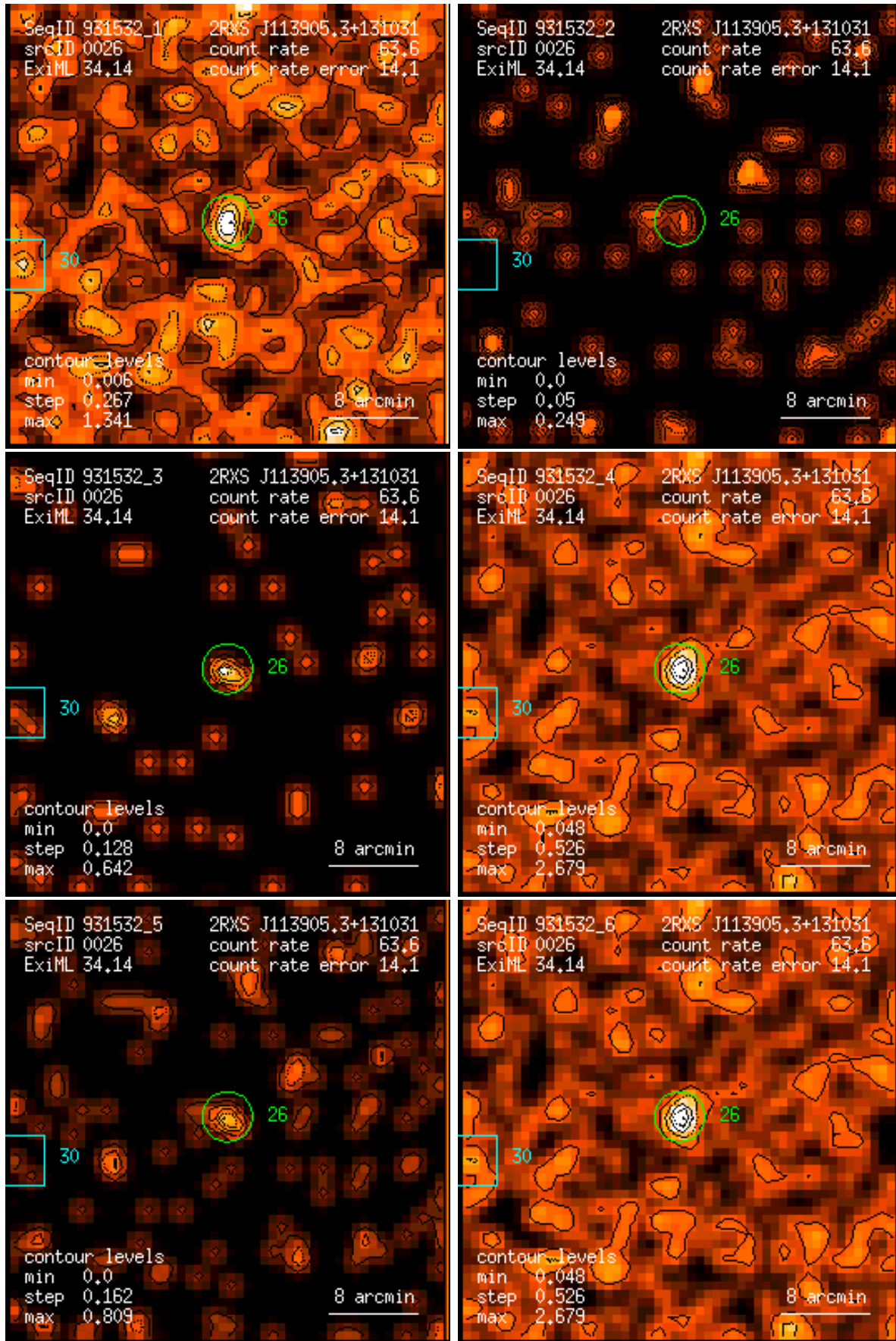
Figure 26: RASS 931532: detection 0026: band rate images, Gaussian filter: (1) PSPC channels 11 – 41, (2) 52 – 90, (3) 91 – 201, (4) 11 – 235, (5) 52 – 201, (6) 11 – 201. Broad band rates in counts/ks. Band rate contour levels in counts/ks/arcmin 2 .
