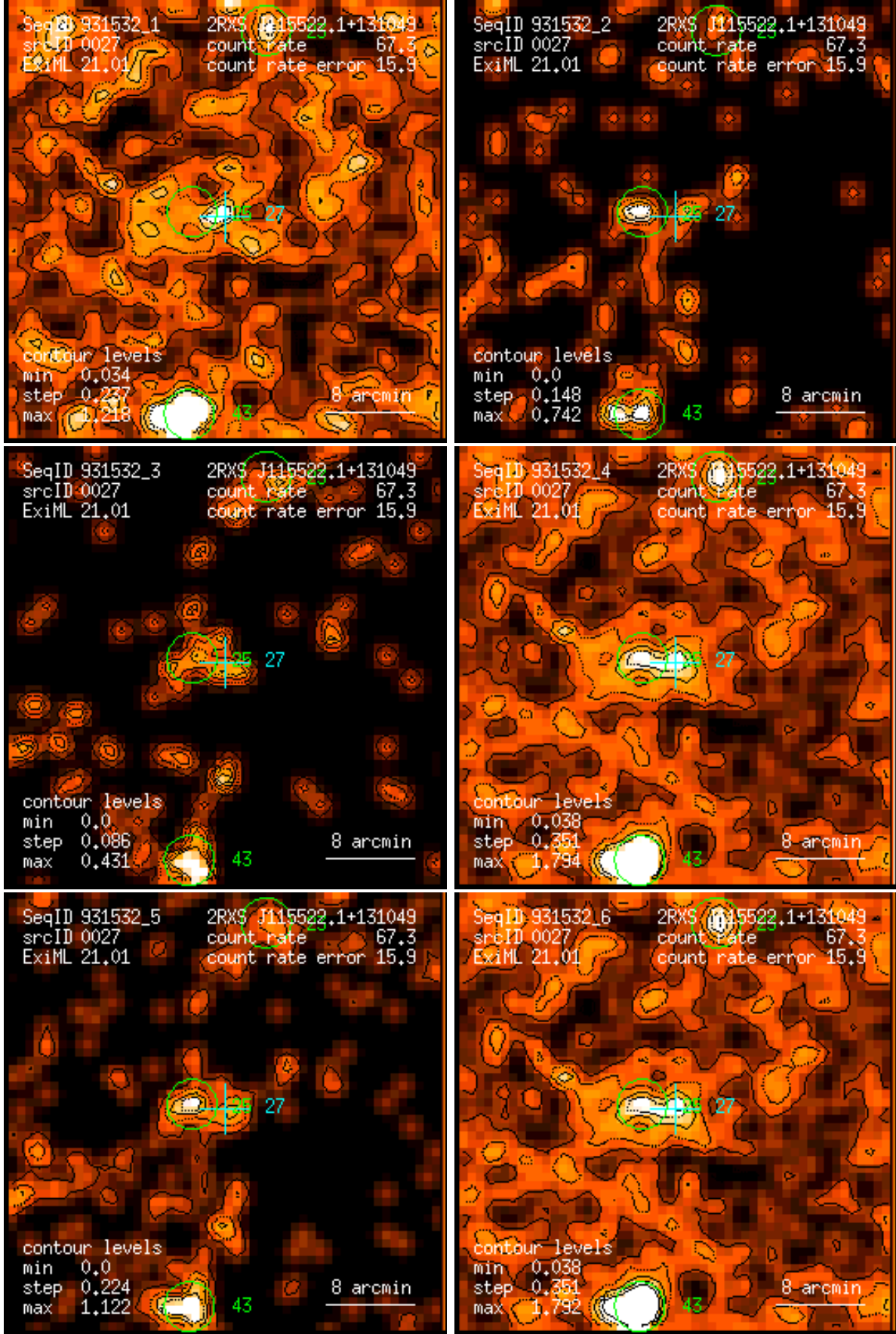
Figure 27: RASS 931532: detection 0027: band rate images, Gaussian filter: (1) PSPC channels 11 – 41, (2) 52 – 90, (3) 91 – 201, (4) 11 – 235, (5) 52 – 201, (6) 11 – 201. Broad band rates in counts/ks. Band rate contour levels in counts/ks/arcmin 2 .
