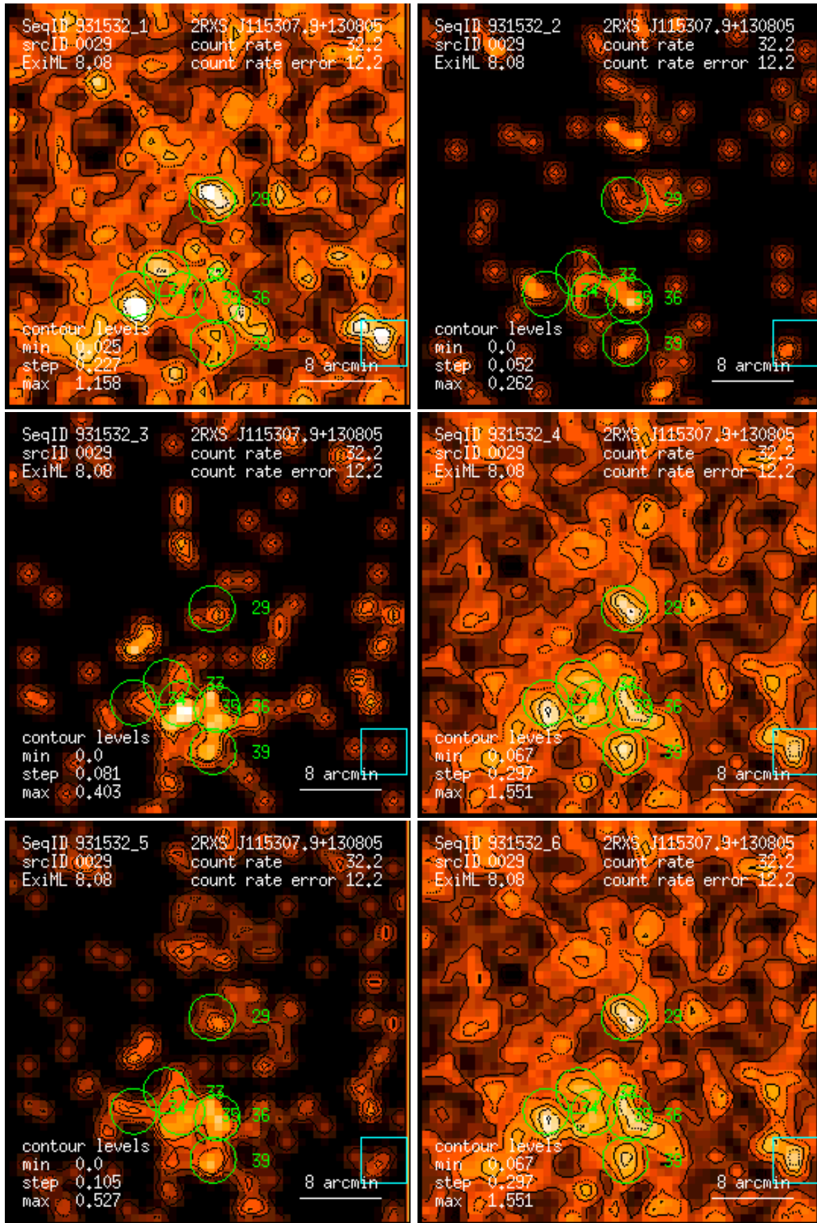
Figure 29: RASS 931532: detection 0029: band rate images, Gaussian filter: (1) PSPC channels 11 – 41, (2) 52 – 90, (3) 91 – 201, (4) 11 – 235, (5) 52 – 201, (6) 11 – 201. Broad band rates in counts/ks. Band rate contour levels in counts/ks/arcmin 2 .
