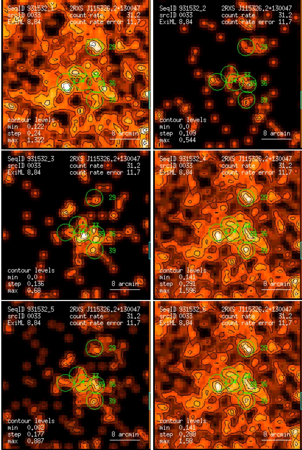
Figure 33: RASS 931532: detection 0033: band rate images, Gaussian filter: (1) PSPC channels 11 – 41, (2) 52 – 90, (3) 91 – 201, (4) 11 – 235, (5) 52 – 201, (6) 11 – 201. Broad band rates in counts/ks. Band rate contour levels in counts/ks/arcmin 2 .
