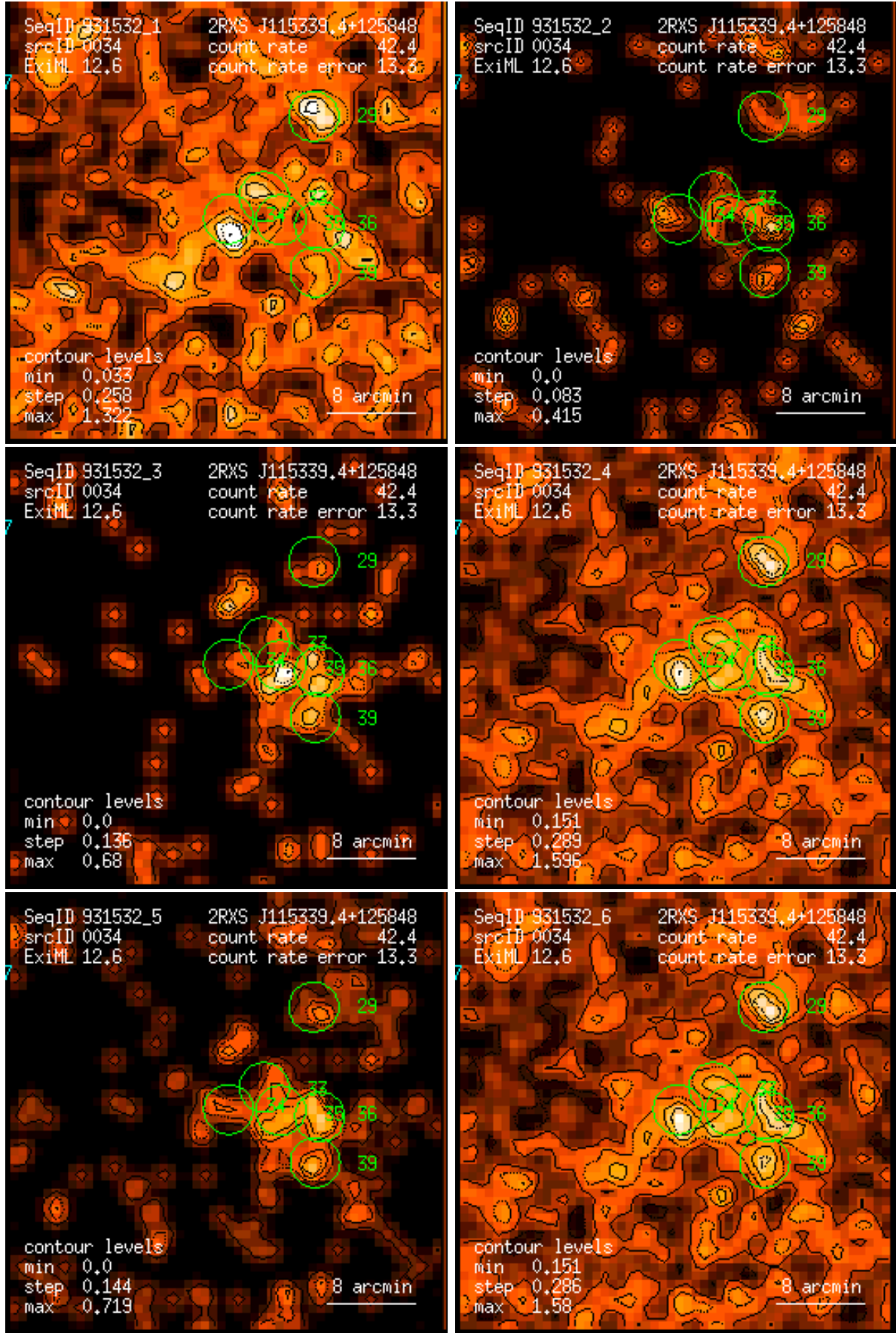
Figure 34: RASS 931532: detection 0034: band rate images, Gaussian filter: (1) PSPC channels 11 – 41, (2) 52 – 90, (3) 91 – 201, (4) 11 – 235, (5) 52 – 201, (6) 11 – 201. Broad band rates in counts/ks. Band rate contour levels in counts/ks/arcmin 2 .
