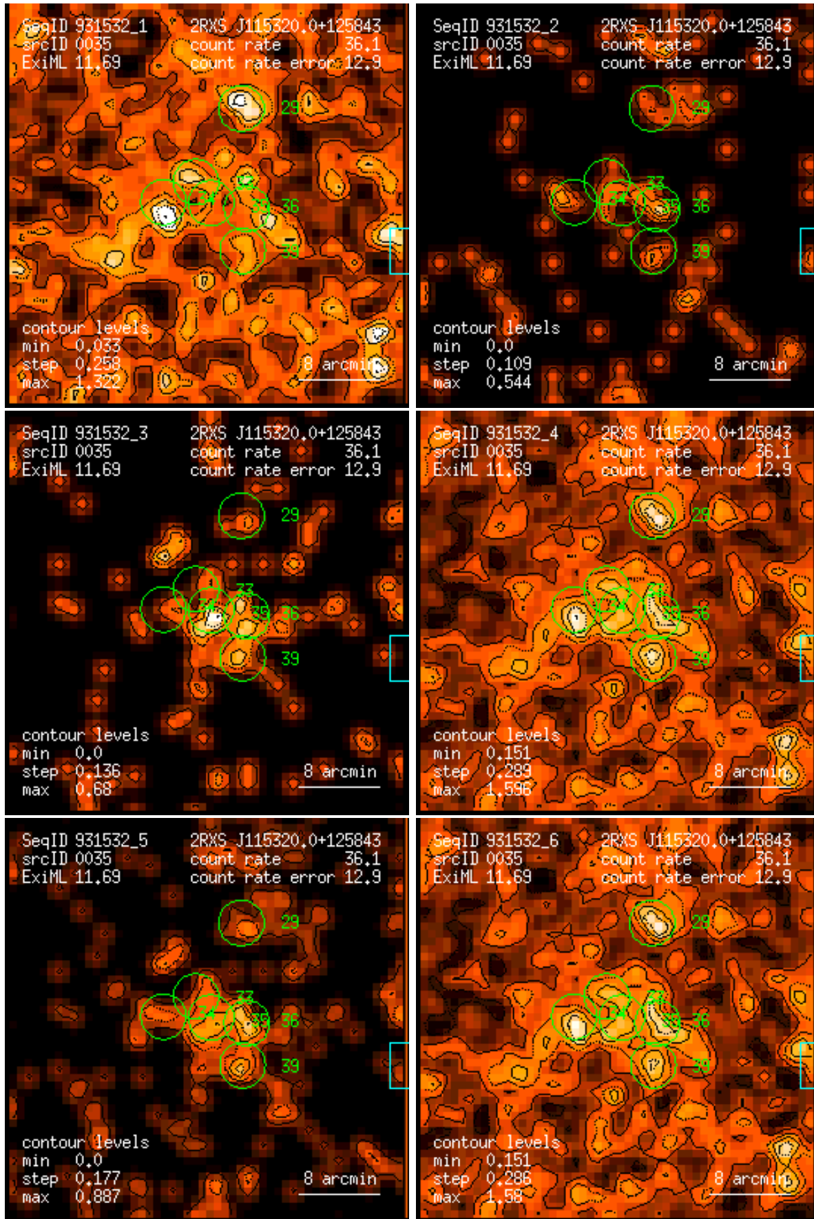
Figure 35: RASS 931532: detection 0035: band rate images, Gaussian filter: (1) PSPC channels 11 – 41, (2) 52 – 90, (3) 91 – 201, (4) 11 – 235, (5) 52 – 201, (6) 11 – 201. Broad band rates in counts/ks. Band rate contour levels in counts/ks/arcmin 2 .
