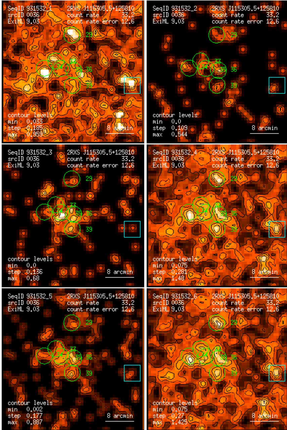
Figure 36: RASS 931532: detection 0036: band rate images, Gaussian filter: (1) PSPC channels 11 – 41, (2) 52 – 90, (3) 91 – 201, (4) 11 – 235, (5) 52 – 201, (6) 11 – 201. Broad band rates in counts/ks. Band rate contour levels in counts/ks/arcmin 2 .
