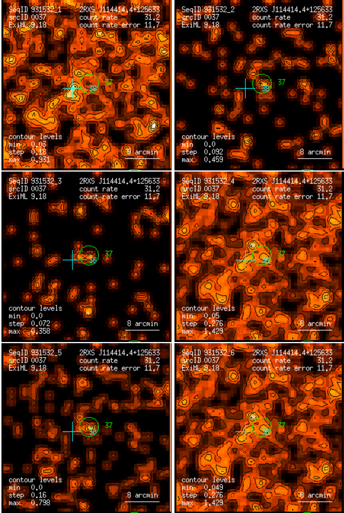
Figure 37: RASS 931532: detection 0037: band rate images, Gaussian filter: (1) PSPC channels 11 – 41, (2) 52 – 90, (3) 91 – 201, (4) 11 – 235, (5) 52 – 201, (6) 11 – 201. Broad band rates in counts/ks. Band rate contour levels in counts/ks/arcmin 2 .
