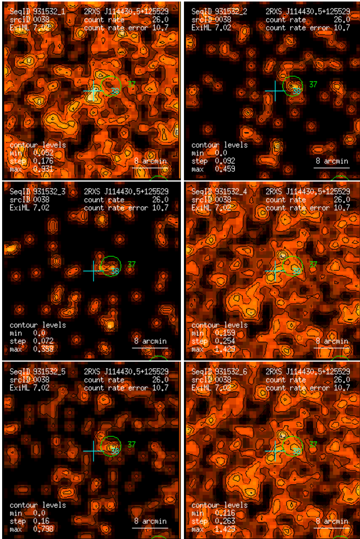
Figure 38: RASS 931532: detection 0038: band rate images, Gaussian filter: (1) PSPC channels 11 – 41, (2) 52 – 90, (3) 91 – 201, (4) 11 – 235, (5) 52 – 201, (6) 11 – 201. Broad band rates in counts/ks. Band rate contour levels in counts/ks/arcmin 2 .
