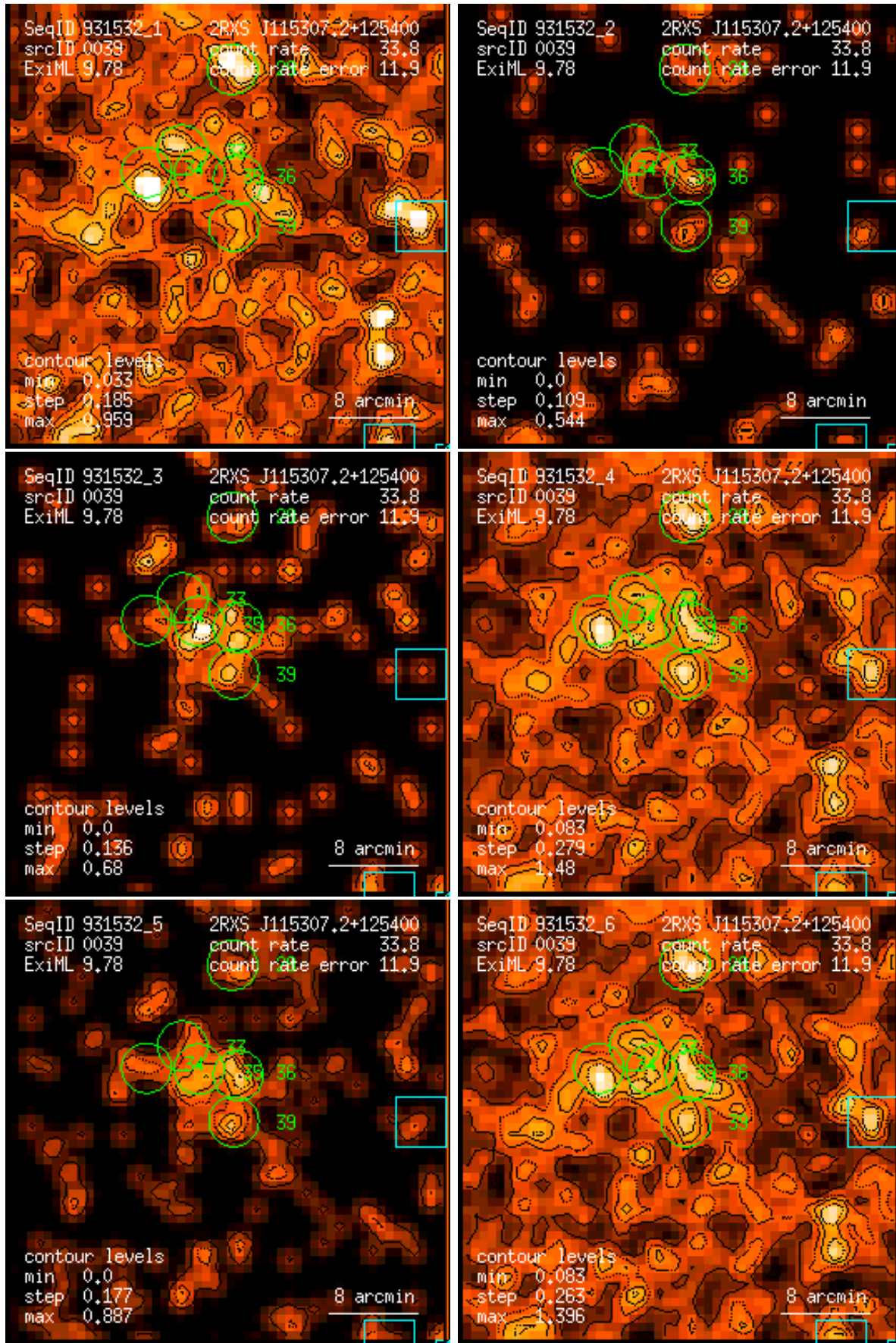
Figure 39: RASS 931532: detection 0039: band rate images, Gaussian filter: (1) PSPC channels 11 – 41, (2) 52 – 90, (3) 91 – 201, (4) 11 – 235, (5) 52 – 201, (6) 11 – 201. Broad band rates in counts/ks. Band rate contour levels in counts/ks/arcmin 2 .
