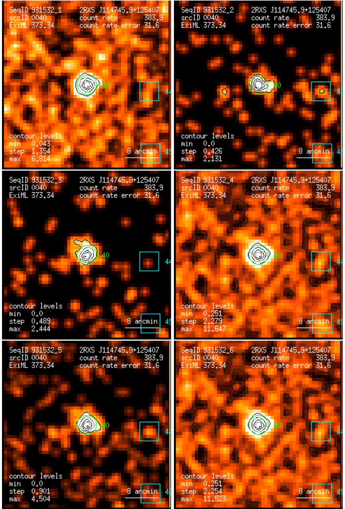
Figure 40: RASS 931532: detection 0040: band rate images, Gaussian filter: (1) PSPC channels 11 – 41, (2) 52 – 90, (3) 91 – 201, (4) 11 – 235, (5) 52 – 201, (6) 11 – 201. Broad band rates in counts/ks. Band rate contour levels in counts/ks/arcmin 2 .
